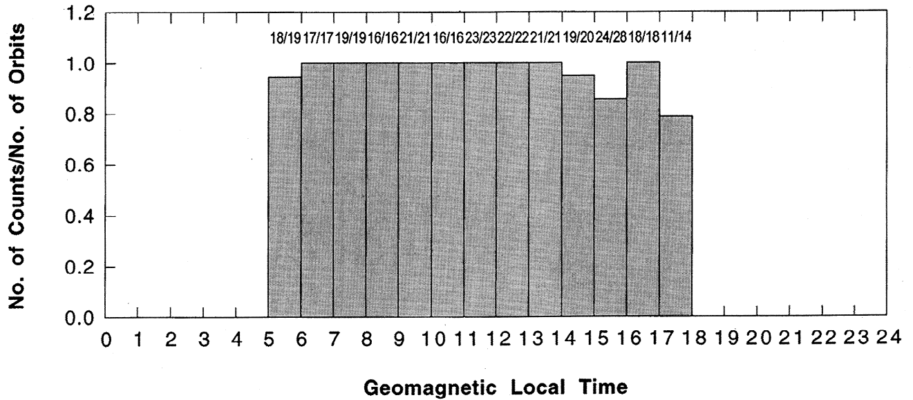
Figure 3. Occurrence frequency of northern dayside PCBL waves as a function of local time. The polar cap boundary layer waves are present on the dayside 96% of the time (0500-1800 LT). The statistics are listed at the top.
