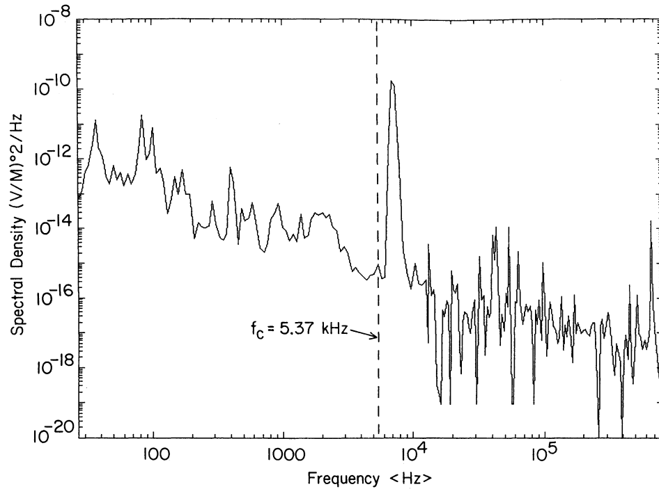
Figure 5. Power spectral density versus frequency for an \sim 32 -s period beginning at 0953:52.839 UT. The dashed line indicates the electron cyclotron frequency. The spectral density of the EEC wave near f_c corresponds to an electric field intensity of \sim 0.112 \text{ mV m}^{-1} .
