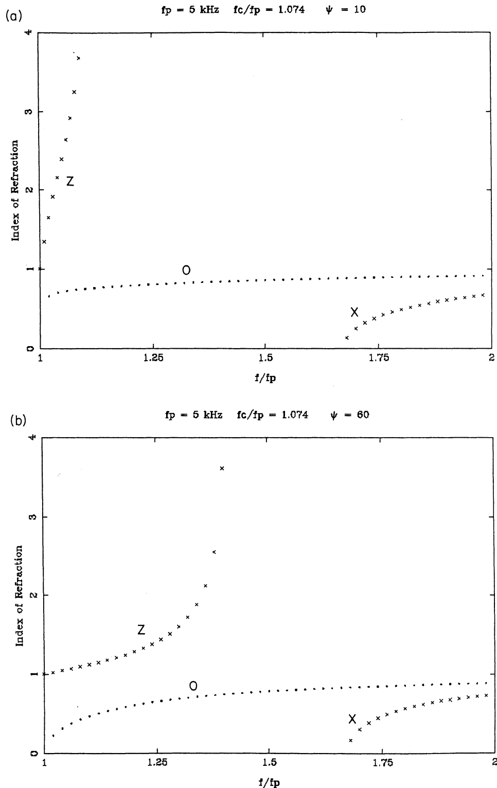
Figure 7. Theoretical cold plasma indices of refraction for a plasma with f_p = 5 \text{ kHz} and f_c = 5.37 \text{ kHz} (for 0954:03 UT) for wave normal angles of (a) 10^\circ and (b) 60^\circ . The wavemodes are indicated on the curves.
