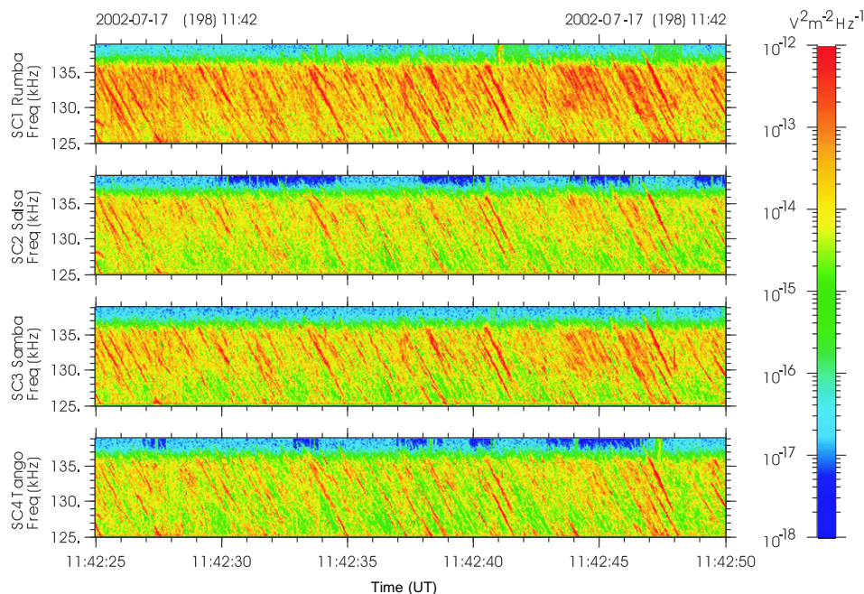
Fig. 6. Spectrogram of the waves observed on all four Cluster satellites on 17 July 2002 over a 25 s time interval in the frequency range of 125.5–136 kHz (the filter cut-off) showing striated Auroral Kilometric Radiation (negative sloped stripes persisting across much of the frequency range) that correlates well across all four satellites. These remotely sensed striations are thought to be tracers of ion holes propagating in the auroral acceleration region.
