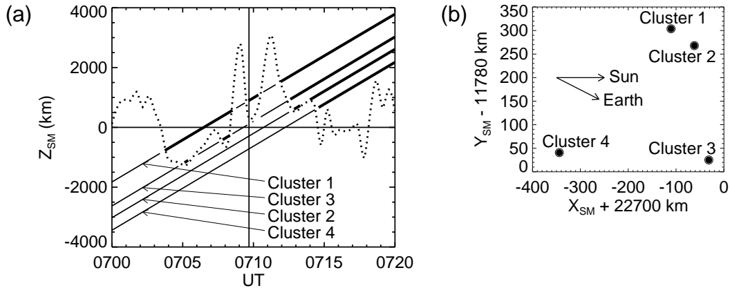
Fig. 3. (a) Four oblique lines represent changes of the sign of S_{||} / \sigma S_{||} along the orbit of the four Cluster spacecraft plotted in the Z_{SM} coordinate as a function of time; the dotted line is the estimated central position of the chorus source region (see text). The horizontal solid line is the magnetic equator, the vertical solid line shows the moment when the center of mass of the four spacecraft crosses the equator. (b) Positions of the spacecraft in the equatorial plane. Arrows show the earthward and the sunward directions.
