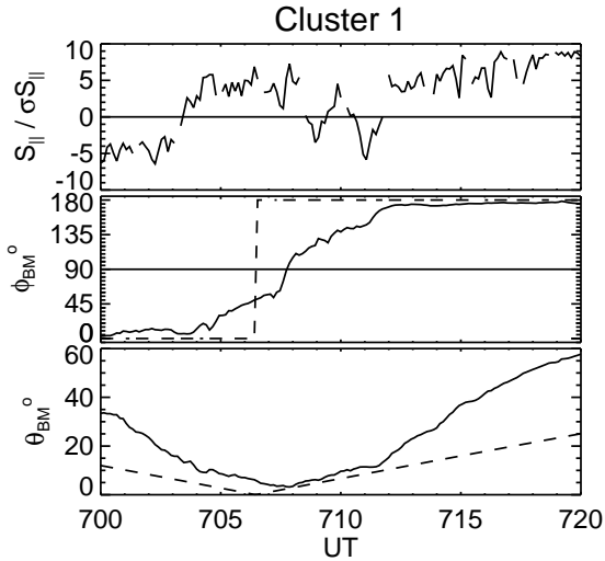
Fig. 8. Comparison of the normalized parallel component of the Poynting flux S_{\parallel} / \sigma S_{\parallel} with the direction of the ambient magnetic field \mathbf{B}_0 expressed by azimuth \phi_{BM} measured around the Z_{SM} axis from the plane of the local meridian, and by the angle \theta_{BM} between the \mathbf{B}_0 direction and the Z_{SM} axis. Solid line corresponds to the onboard measurement, dashed line shows the dipole model.
