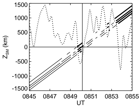
Fig. 6. The same as in Fig. 3 for measurements recorded on 18 April 2002.
