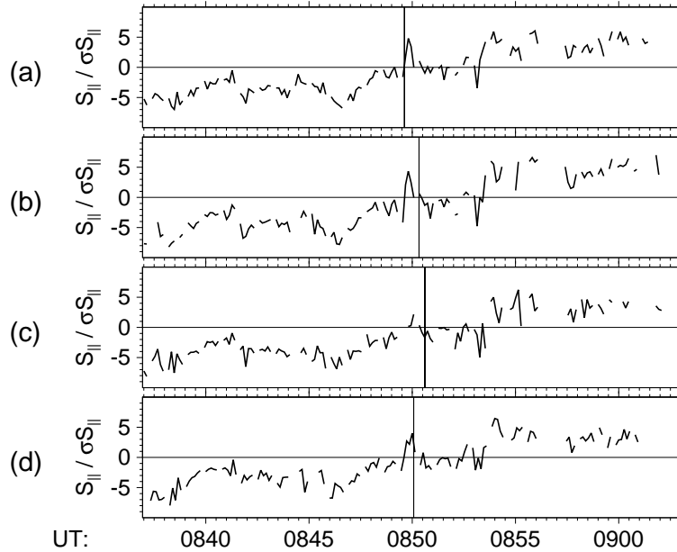
Fig. 5. The same as in Fig. 2 but for measurements recorded on 18 April 2002.
