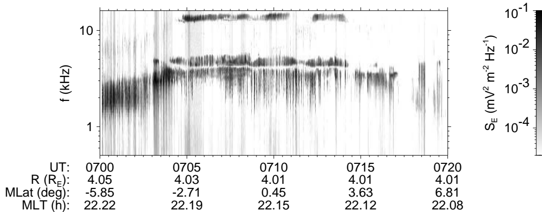
Fig. 1. Power-spectrogram of the electric field measured onboard Cluster 3 on 31 March 2001. Position of the spacecraft is given on the bottom. R - radial distance in Earth radii; Mlat - magnetic dipole latitude in degrees; MLT - magnetic local time in hours.
