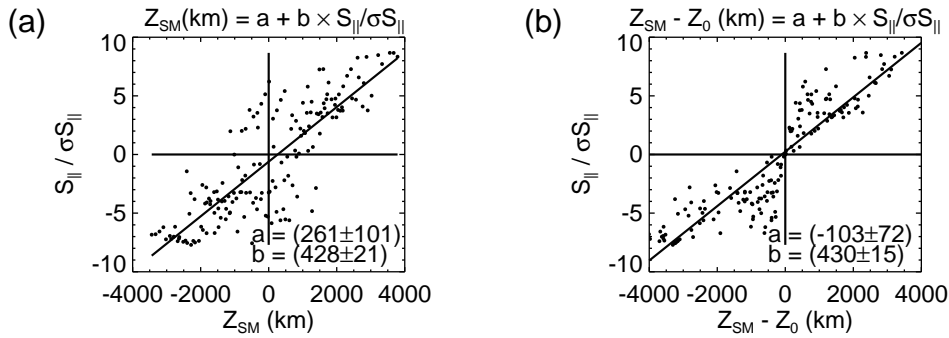
Fig. 4. (a) Linear fit to the obtained S_{\parallel} / \sigma S_{\parallel} values as a function of the Z_{SM} coordinate. (b) The same but using the difference of the Z_{SM} coordinate and the estimated central position of the source.
