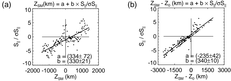
Fig. 7. The same as in Fig. 4 but for the data recorded on 18 April 2002.
