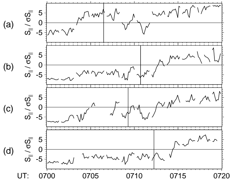
Fig. 2. Parallel component of the Poynting vector normalized by its standard deviation. Panels (a)–(d) show the results for Cluster 1–4, respectively. Vertical line in each panel indicates the moment when the given spacecraft encounters the magnetic equatorial plane (zero magnetic latitude). Dipole model is used.
