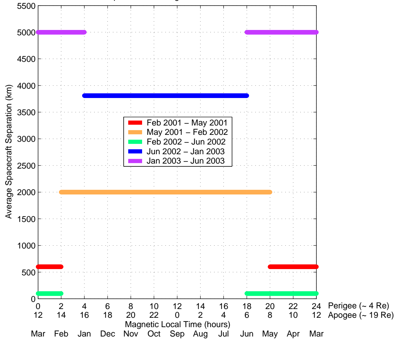
Cluster Separations vs. Magnetic Local Time and Month
