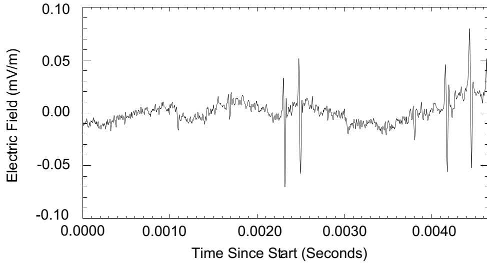
a) Cluster WBD Time Series
