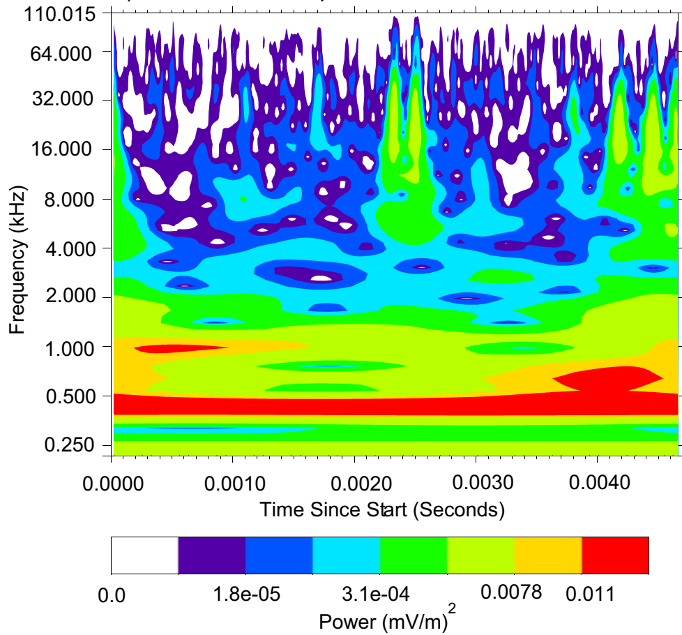
b) Wavelet Power Spectrum
