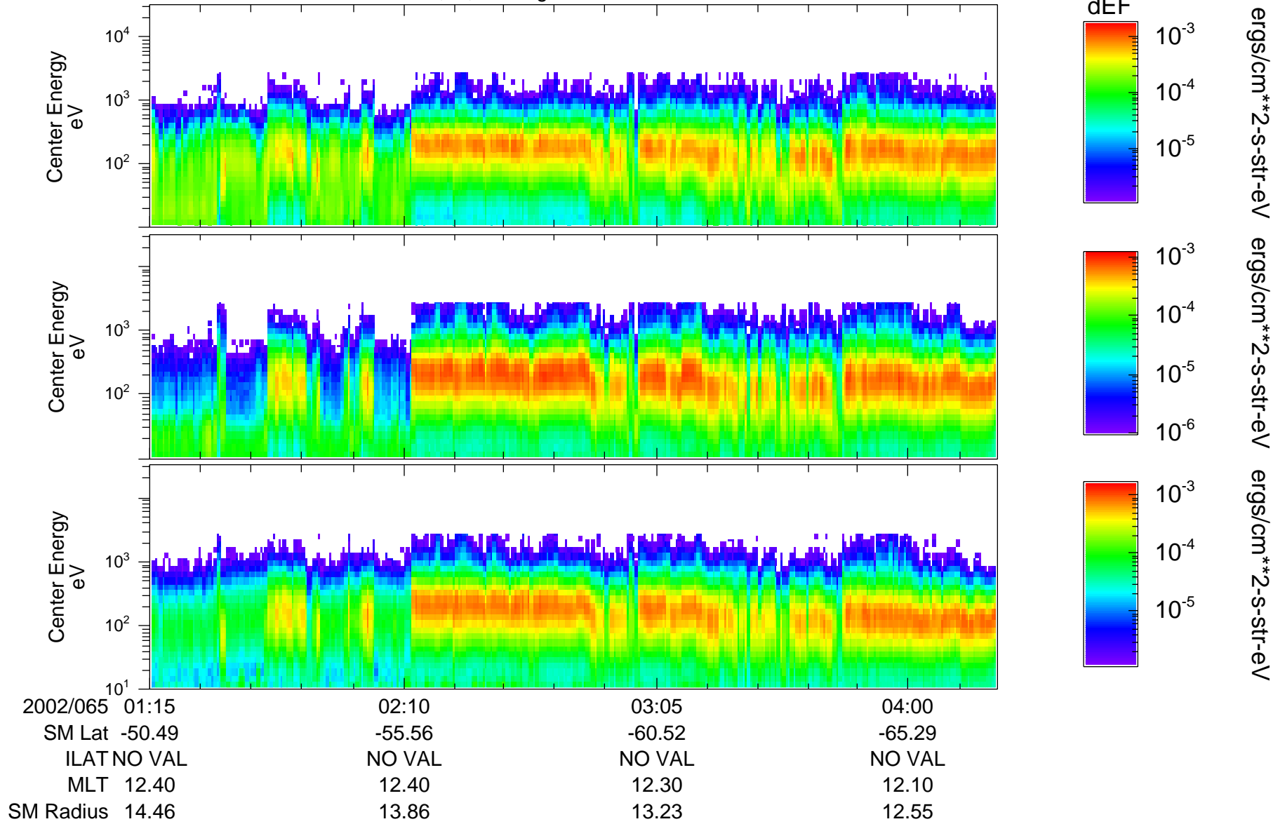
Cluster 4 PEACE Electrons at 0,90,180 deg V wrt B
