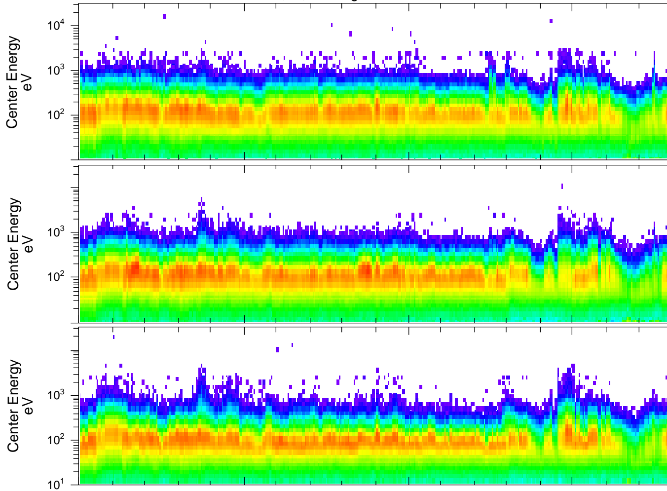
Cluster 4 PEACE Electrons at 0,90,180 deg V wrt to B
