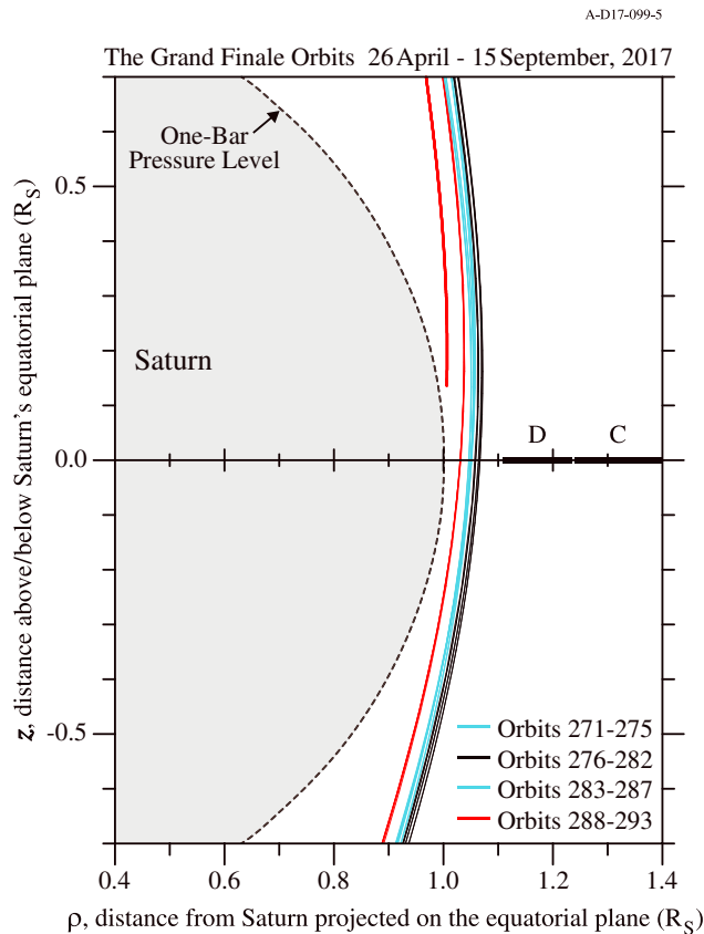
Figure 1. A meridional plot in cylindrical coordinates showing the tightly grouped Cassini trajectories for all of the Grand Finale orbits. The trajectories are shown in four time-sequenced groups and color coded according to the altitude of Cassini at closest approach.
