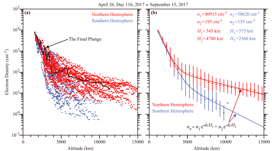
Figure 4. The altitude distribution of the Radio and Plasma Wave Science electron density profiles for all of the Grand Finale orbits. Panel (a) shows the density measurements for the northern hemisphere in red, the density measurements for the southern hemisphere in blue, and the density measurements for Cassini’s plunge into Saturn’s upper atmosphere (part of the northern data set) as a solid black line. There is very little spread at the lowest altitudes for both hemispheres, but the variability increases at higher altitudes. The north-south asymmetry, attributed to the reduced ionization and electron density depletions in the southern hemisphere from the ring shadow effect, is evident in the divergence in the north and south distributions above 3,000 km. Panel (b) shows the same data averaged in altitude bins of 500 km and a classic ionospheric density distribution with two ionospheric layers. The fit of the scale height model to the averaged data uses a two-part exponential equation: n_e = n_1 e^{-h/H_1} + n_2 e^{-h/H_2} , where subscript 1 refers to the ionospheric layer at the lower altitudes and subscript 2 refers to the ionospheric layer at the higher altitudes.
