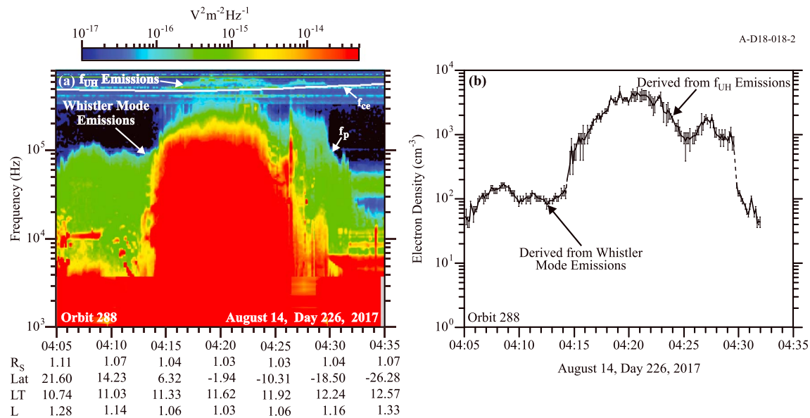
Figure 2. Panel (a) is a color Radio and Plasma Wave Science spectrogram for orbit 288 illustrating both the broadband whistler mode emissions and the narrowband upper hybrid resonance ( f_{UH} ) emissions. Electron density measurements are obtained from the wave propagation characteristics of these plasma wave modes. Panel (b) shows the electron density measurements derived from these plasma wave spectral features.
