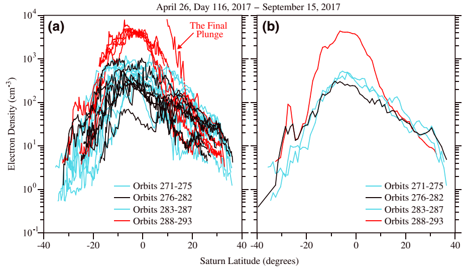
Figure 3. Panel (a) shows the latitudinal distributions of the Radio and Plasma Wave Science electron density measurements for all of the Grand Finale orbits. The latitudinal electron density profiles are color coded according to the altitude of Cassini at closest approach. These latitudinal profiles show strong variability from orbit to orbit, up to 2 orders of magnitude, as well as a significant north-south asymmetry due, in part, to the ring shadow effect in the southern hemisphere. Panel (b) shows the electron density measurements for the four groupings of the Grand Finale orbits averaged in latitude bins of 2^\circ . The averaged latitudinal electron density profiles show a strong altitude dependence within 10^\circ of the ring plane.
