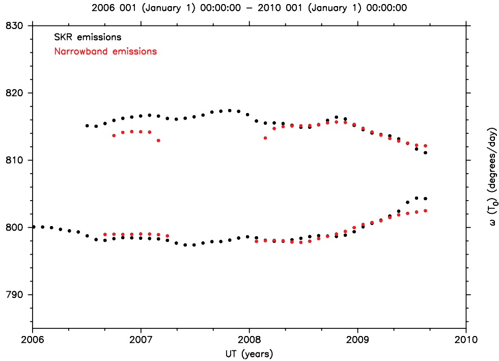
Figure 5: SKR vs. narrowband modulation periods from 2006 to 2010. The red dots represent the periods of Saturn narrowband emissions. The black dots represent the periods of SKR given by Gurnett et al. [2009a].
