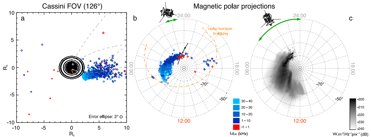
Figure 2. (a) Location of radio sources in Cassini’s field of view, or FOV, and (b) magnetically projected down to the planet. The radio data selection is described in the auxiliary material. The time-frequency interval is restricted to [0812,0912] UT (source region) and [f_{ce} - 1 \text{ kHz}, f_{ce} + 40 \text{ kHz}] (highest resolution). Crosses (diamonds) refer to directions of arrival that cross (do not cross) their associated isosurface f = f_{ce} [Cecconi et al., 2009]. Most of the frequencies (plotted in blue scale for increasing ranges of f - f_{ce} ) correspond to distant sources, clustered along high-latitude magnetic field lines in panel a (dashed, with footprint coordinates LT_B = [0400, 0600] and \lambda_B = [-80^\circ, -75^\circ] ), quantitatively identified on the dawnside in Figure 2b. Frequencies plotted in red ( f \leq f_{ce} + 1 \text{ kHz} ) reveal local sources, detected through the entire observation plane in Figure 2a, and mapping the ionosphere along field lines crossed by Cassini in panel b, the green (black) line showing the projected spacecraft trajectory for [0812,0912] UT ([0600,1100] UT). (c) Radio map [Lamy et al., 2009] integrated along the extended time interval [0700,1100] UT and frequency range [7,1000 kHz]. The global distribution of the footprints of field lines supporting SKR sources follows an unusual spiral shape, starting from narrow very high latitude \lambda_B = -80^\circ \pm 2^\circ at LT_B = 0100 , then evolving to broad lower latitudes toward noon until \lambda_B = -75 \pm 6^\circ at LT_B = 1300 .
