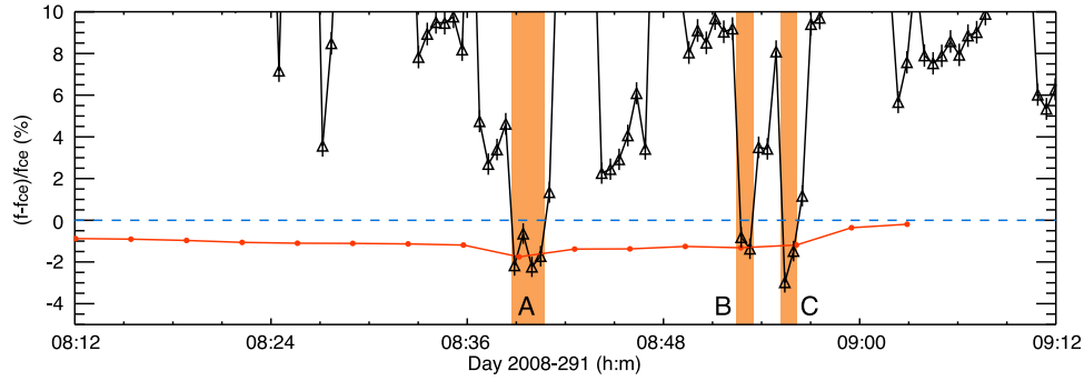
Figure 3. Characteristic frequencies between 0812 and 0912 UT, expressed relatively to f_{ce} . The SKR cutoff frequency f_{cut} , determined with an accuracy of 0.5%, is displayed in black, and f_{ce} , in dashed blue. The red curve refers to the CMI resonance frequency f = f_{ce}/\Gamma computed with hot electrons observed by CAPS under the assumption of perpendicular SKR emission, with an uncertainty less than the size of dots. The linear correlation coefficient between f and f_{cut} , for the 8 measurements f_{cut} \leq f_{ce} observed during events A, B and C, is c = 0.94 .
