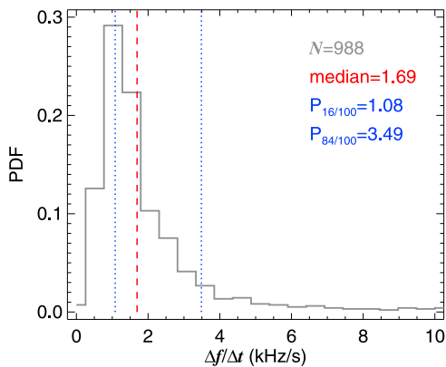
Figure 4. PDF of the sweep rate of risers from 21 October 2001. The dashed line labels the median sweep rate; the dotted lines describe the P_{16/100} and P_{84/100} percentiles.
