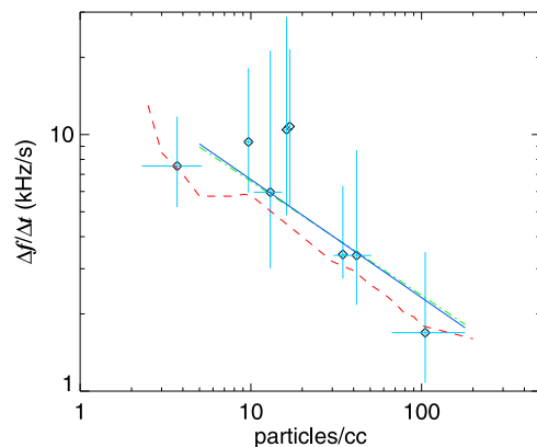
Figure 7. The same as in Figure 6 but on a log-log scale and with a theoretical scaling according to equation (11). The green dashed-dotted line describes a linear fit of the logarithm of the median of risers versus the logarithm of the median plasma density, taking into account measurement errors (\log P_{16/100} - \log P_{84/100})/2 . The blue solid line shows a linear fit of the logarithm of the geometrical average of P_{16/100} and P_{84/100} versus the logarithm of the median plasma density, taking into account the same measurement errors.
