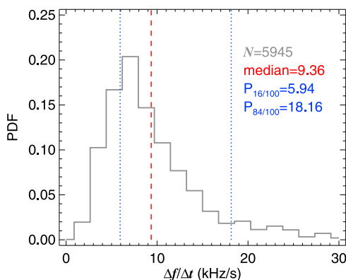
Figure 2. Probability density function (PDF) of the sweep rate of risers measured on 6 December 2003. The dashed line shows the median sweep rate; the dotted lines give the P_{16/100} and P_{84/100} percentiles.
