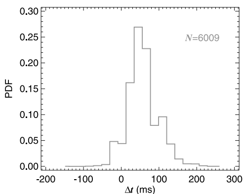
Figure 5. PDF of the duration of chorus elements measured on 6 December 2003. Negative values \Delta t (ms) represent falling tones with negative frequency sweep rates.
