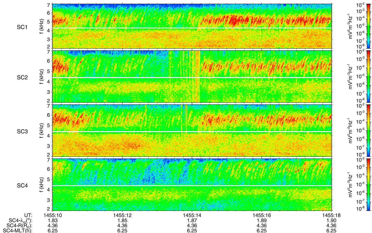
Figure 1. Example of chorus wave packets measured at L = 4.2 on 6 December 2003 by the Cluster satellites 1, 2, 3, and 4. Time and spacecraft position are given on the bottom: UT, universal time; \lambda_m , magnetic dipole latitude; R_E , Earth radius; MLT, magnetic local time. One half of the electron cyclotron frequency (white line) for satellite 1 is 4.3 kHz, for satellite 2 it is 4.4 kHz, for satellite 3 it is 4.3 kHz, and for satellite 4 it is 4.4 kHz.
