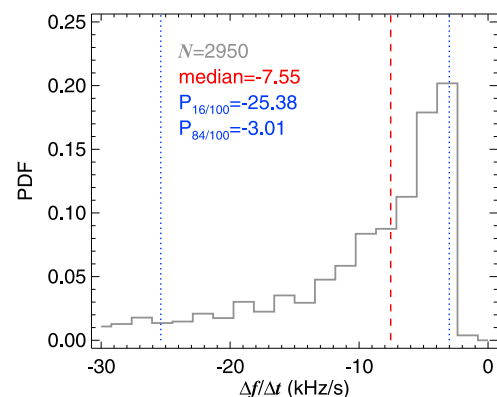
Figure 3. PDF of the sweep rate of fallers from 19 November 2001. The dashed line represents the median sweep rate; the dotted lines give the P_{16/100} and P_{84/100} percentiles.
