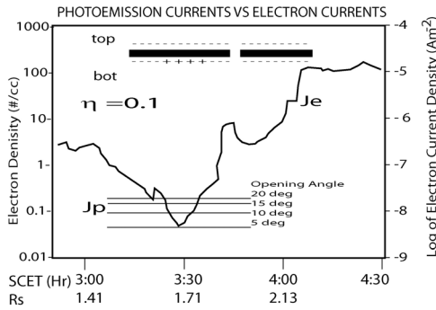
Figure 3. A comparison of the plasma electron currents to the photoemission current. The photoemission currents are presented as a function of opening angle. At locations where J_p > J_e , the sunlit bottom side of the B ring should charge to a positive potential.
