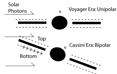
Figure 2. An illustration of the change in ring electrical configuration from Voyager in the early 1980s to Cassini. The opening of the rings allows more photoemission from the bottom side ring, thereby charging it positive.
