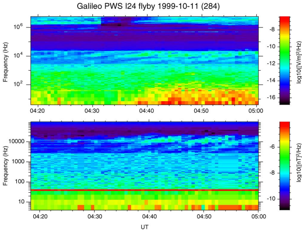
Fig. 3. Same as Fig. 2 but for the upstream I24 flyby. The closest approach occurred at 04:33:03 UT.
