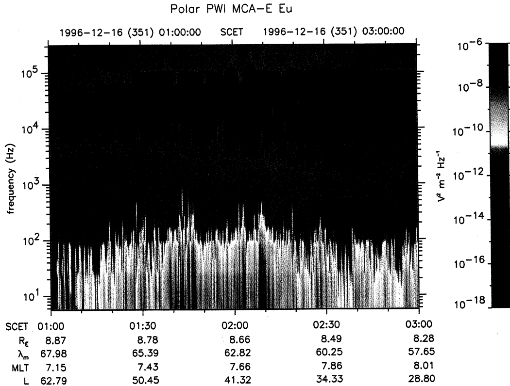
Plate 2. A long-duration PCBL wave event detected at local dawn on December 16, 1996.
