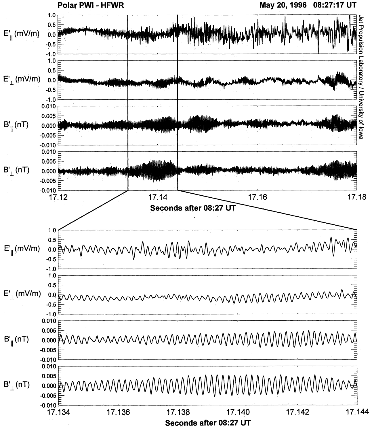
Figure 16. Electromagnetic whistler-mode waves at \sim 4.9 \text{ kHz} . These emissions were detected near local noon. The emissions are most probably “auroral hiss” detected at lower altitudes.
