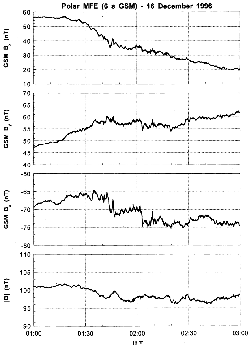
Figure 13. The magnetic field for the event of Plate 2. The strong field gradient regions and strong wave intensity regions are coincident, as in the case in Plate 1 and Figure 7.
