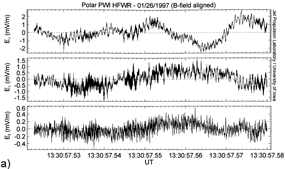
Figure 17. (a) Examples of high-frequency \sim 10 -kHz electric waves sporadically superposed on top of \sim 1 -kHz electric oscillations. (b) The power spectra for the same interval. The “ \sim 1 kHz waves” in actuality cover a broad frequency range from \sim 7 \times 10^2 to \sim 3 \times 10^3 Hz. The 10-kHz waves form a narrow peak. The dominant power of the latter waves is present in E_{\perp} .
