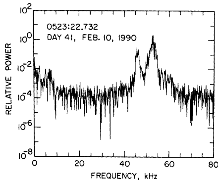
Figure 7. The spectrum of the waveform from Figure 4b. Note the weak low-frequency signals located from a few hundred hertz to approximately 9 kHz. These low-frequency signals are suggestive of the low-frequency ion acoustic waves predicted by parametric decay.
