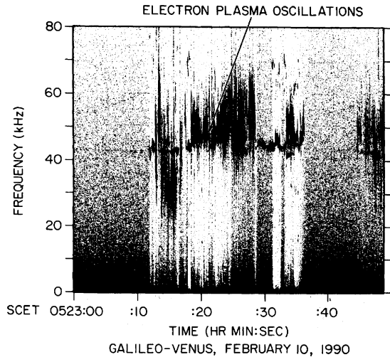
Figure 3. A high-resolution frequency-time spectrogram of the Langmuir waves. The Langmuir waves show temporal structure down to the resolution of the Fourier transform (66.67 ms). Large upshifts and downshifts in the emission frequency compared to the plasma frequency ( \sim 43 kHz) are also observed. (From Gurnett et al. [1991].)
