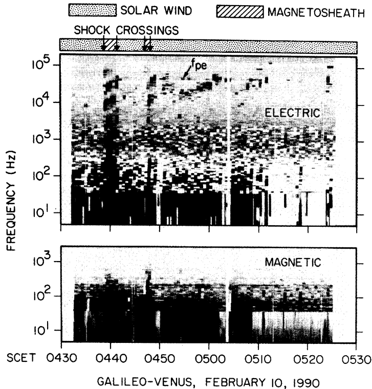
Figure 2. A frequency-time spectrogram of the electric and magnetic field intensities measured by the medium- and low-frequency spectrum analyzers. Four bow shock crossings and the plasma region the spacecraft was in are shown at the top of Figure 2. The Langmuir waves can be most easily seen after the last bow shock crossing, in the frequency band 10 to 50 kHz of the electric field spectrum. (From Gurnett et al. [1991].)
