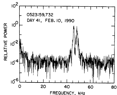
Figure 5. The spectrum of the waveform from Figure 4d. The two distinct signals at approximately 45.5 and 48.3 kHz are evidence that the beat-type waveforms are caused by two waves of comparable amplitude and slightly different frequency beating with each other.
