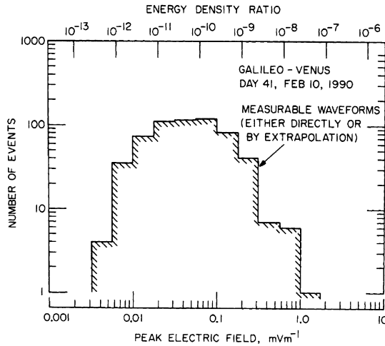
Figure 6. The number of waveform blocks as a function of the peak electric field strength.
