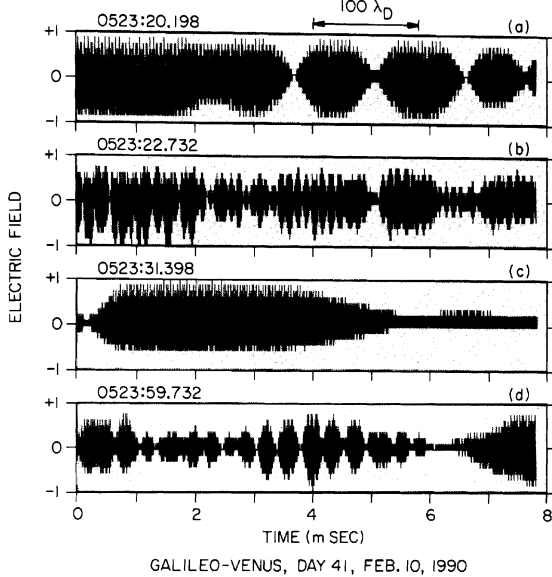
Figure 4. A sampling of the Langmuir emission electric field waveforms. Note the considerable temporal structure down to timescales of 0.15 ms.
