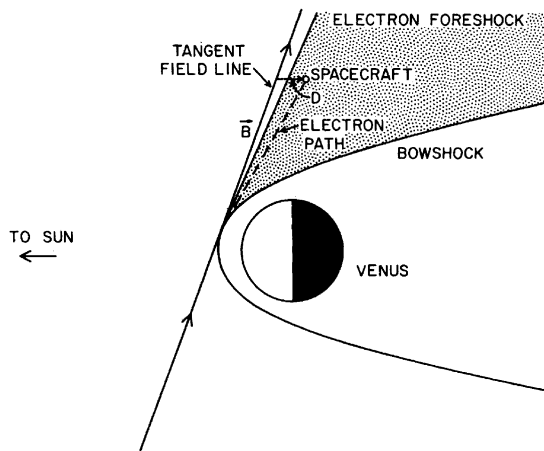
Figure 1. A sketch of the electron foreshock region of Venus. Electrons streaming from the bow shock along the magnetic field lines are convected downstream by the solar wind. These electron beams generate Langmuir waves by the beam-plasma instability. The depth parameter D is defined as the distance from the tangent magnetic field line to the spacecraft.
