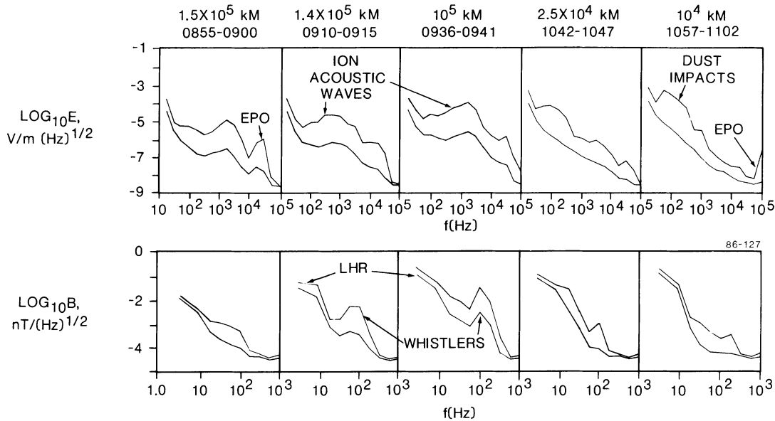
Fig. 3. Characteristic peak and average E and B wave spectra measured as ICE moved inbound from the solar wind (0855–0900) to Giacobini-Zinner closest approach (1102). Here LHR represents the lower hybrid resonance emission and EPO represents electron plasma oscillations
