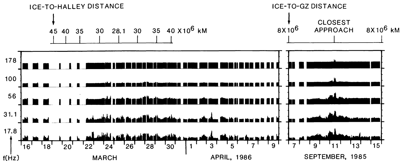
Fig. 6. Low frequency B-field waves observed during closest approach to comets Halley and Giacobini-Zinner
