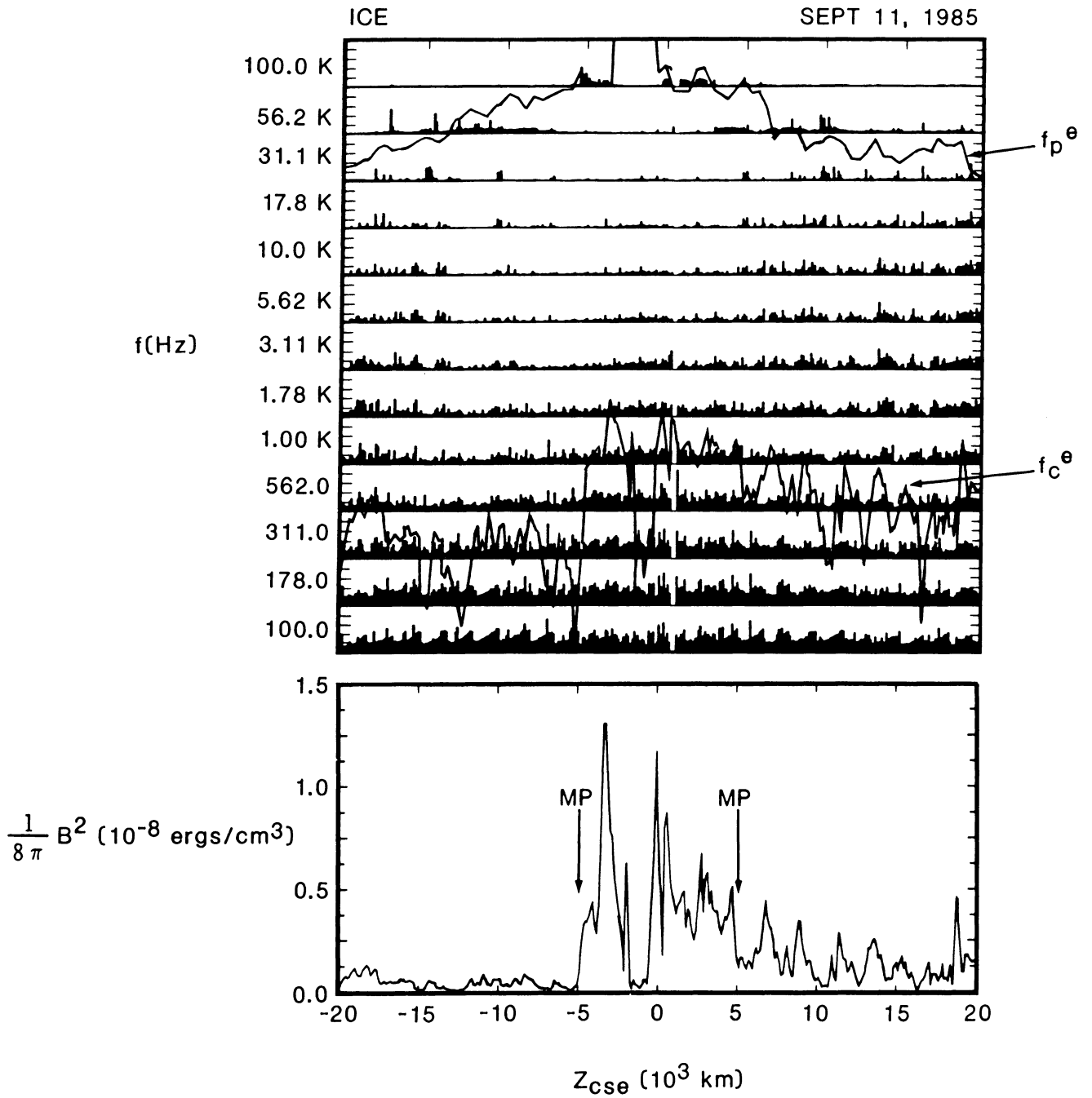
Fig. 5. B-field magnitude and 13-channel E-field wave amplitudes for the ICE crossing of the Giacobini-Zinner plasma tail
