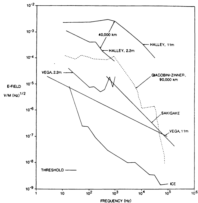
Fig. 8. Plasma wave spectra from Halley (Vega-1 and -2) and Giacobini-Zinner (ICE), together with E-field threshold curves for the comet plasma wave instruments
