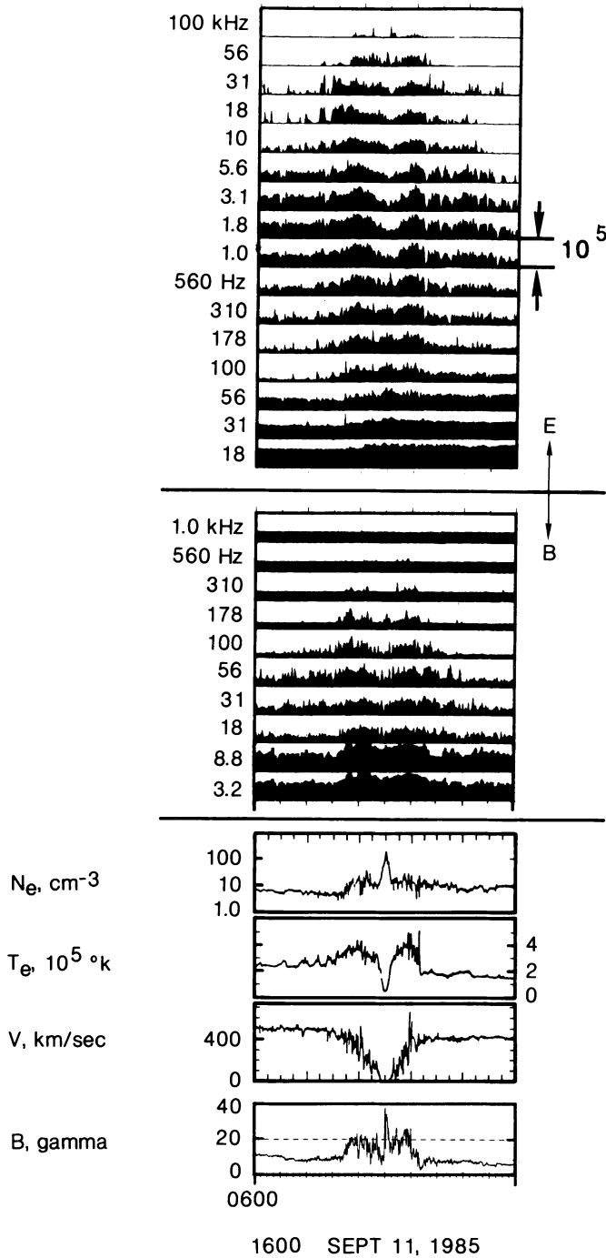
Fig. 2. Summary of plasma wave amplitude data, plasma parameters and B-field profile for the ICE encounter with comet Giacobini-Zinner
