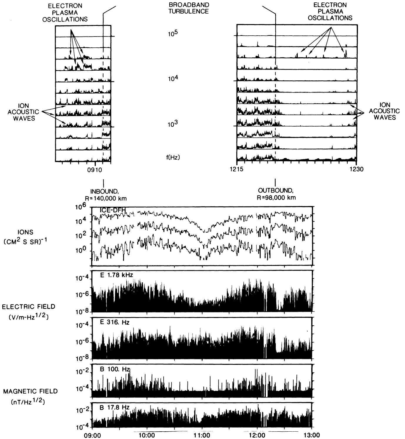
Fig. 4. Bottom: Unaveraged wave profiles in four channels, along with energetic particle fluxes. Top: Unaveraged profiles for all 16 E-field channels. The vertical dashed lines mark the events with collisionless bow shock wave characteristics
