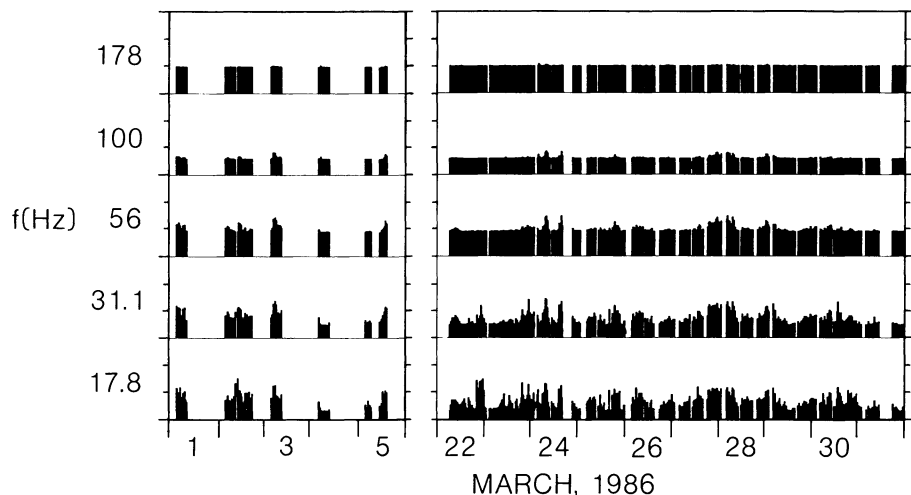
Fig. 6. Low frequency B-field waves observed during closest approach to comets Halley and Giacobini-Zinner
