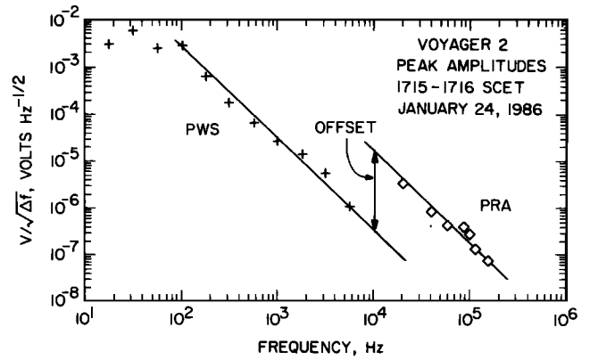
Fig. 7. A comparison of the voltage spectrums detected by the plasma wave (PWS) and radio astronomy (PRA) instruments. The offset is believed to be caused by the different mode of electric field detection used by the two instruments (dipole for PWS and monopole for PRA).
