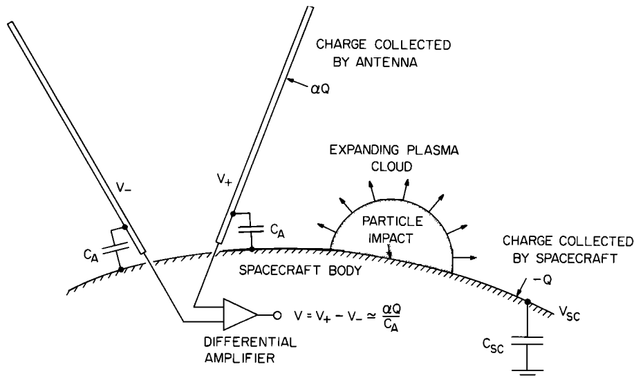
Fig. 6. A schematic illustration of the model used to analyze the voltage produced by an impact. Charge released by the impact is collected by the antenna, \alpha Q , and by the spacecraft body, -Q . These charges produce voltage pulses of amplitudes \alpha Q/C_A on the antenna and -Q/C_{sc} on the spacecraft body. Because the plasma wave instrument operates as a differential system, it does not respond to the voltage pulse on the spacecraft body.
