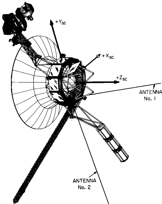
Fig. 1. A sketch of the Voyager spacecraft showing the mounting of the two antenna elements and the spacecraft coordinate system used in the analysis.
