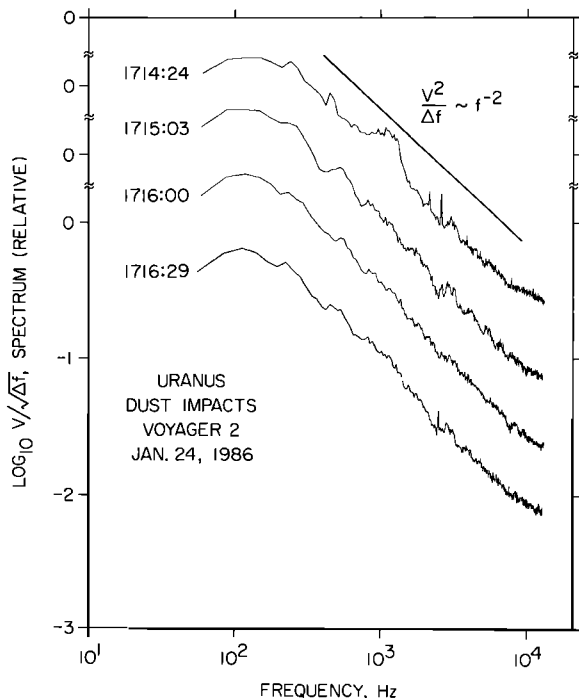
Fig. 5. Selected frequency spectra of the broadband waveform data. The f^{-2} voltage spectrum is believed to be an instrumental effect caused by the square-wave-like waveform that occurs during the recovery phase (see Figure 4).
