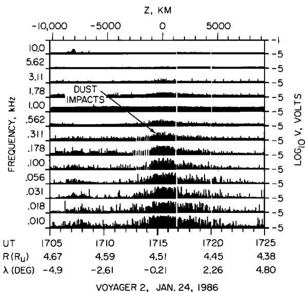
Fig. 3. The voltages measured by the 16-channel spectrum analyzer near the equatorial plane. The very intense broadband noise observed near the equator crossing ( z = 0 ) is caused by particles hitting the spacecraft.
