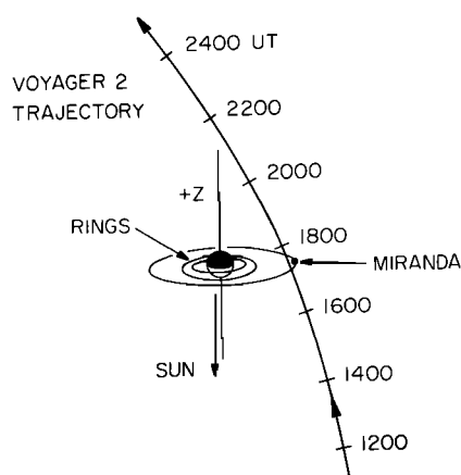
Fig. 2. The trajectory of the Voyager 2 spacecraft in the orbital plane. The spacecraft crossed the equatorial plane outside the visible ring system and inside the orbit of Miranda.
