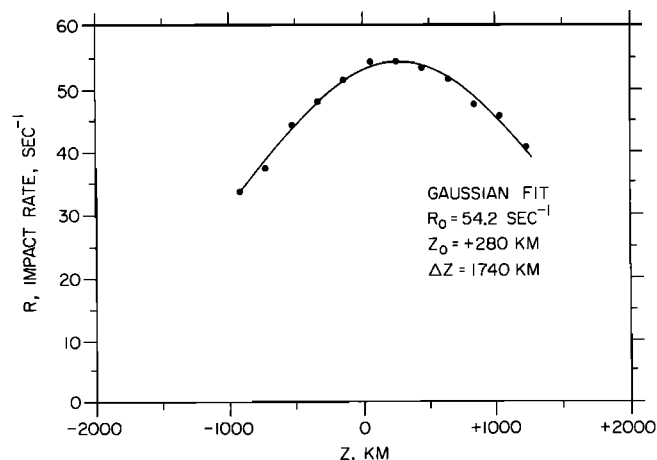
Fig. 8. The impact rate R as a function of the distance z from the equatorial plane and the best fit Gaussian profile (solid line).
