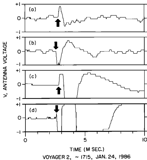
Fig. 4. A series of broadband waveforms of the particle impact noise. Note that both positive and negative polarities occur.
