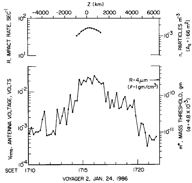
Fig. 9. The impact rate R and rms antenna voltages V_{rms} can be analyzed to give the number density n and mass threshold m^* . These quantities are shown by the scales on the right.
