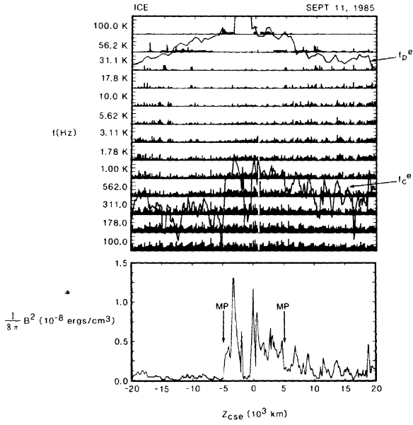
Figure 5. B-field magnitude and 13 channel E-field wave amplitudes for the ICE crossing of the Giacobini-Zimmer plasma tail.
