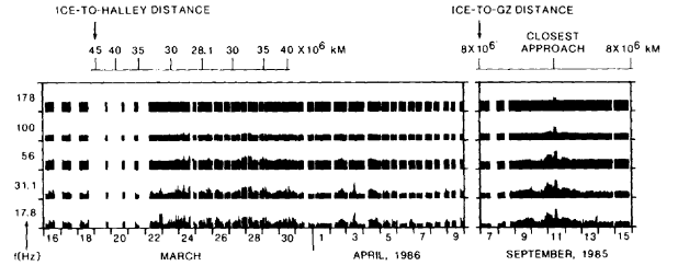
Figure 6. Low frequency B-field waves observed during closest approach to comets Halley and Giacobini-Zimmer.
