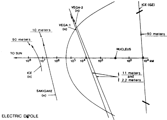
Figure 1. Projected flyby trajectories for the comet encounter spacecraft with on-board wave instruments. The nominal Halley bow shock curve is shown; for Giacobini-Zinner the heavy arcs on the ICE(GZ) plot depict the shock crossing distances. The underlined numbers give the tip-to-tip antenna lengths for the electric dipoles.
