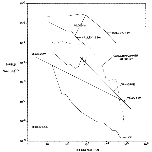
Figure 8. Plasma wave spectra from Halley (VEGA 1 and 2) and Giacobini-Zimmer (ICE), together with E-field threshold curves for the comet plasma wave instruments.
