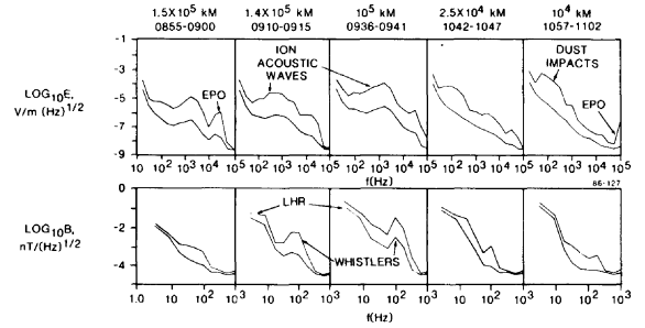
Figure 3. Characteristic peak and average E and B wave spectra measured as ICE moved inbound from the solar wind (0855-0900) to Giacobini-Zinner closest approach (1102).
