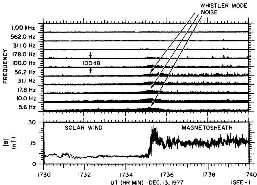
Fig. 1. Typical observations of whistler mode noise at the bow shock [from Tokar et al. , 1984]. The figure depicts data obtained with the ISEE 1 plasma wave experiment and the magnetic field experiment. The top panel shows the wave magnetic fields in 10 frequency channels while the bottom panel illustrates the magnetometer data. The magnetic ramp defining the shock transition region is clearly visible, as is the large-amplitude whistler mode noise at the shock. The noise is most intense within the shock transition region and extends into the upstream solar wind and downstream magnetosheath.
