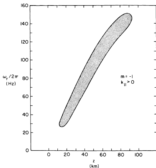
Fig. 4. The unstable frequencies as a function of shock penetration for the model distribution and generation via the normal cyclotron resonance. It is usually true that for a given frequency a wide range of wave normal angles is unstable. The increase in frequency with increasing z is due to the fact that the normal cyclotron resonance velocity must remain in regions of large anisotropy in F(z) .
