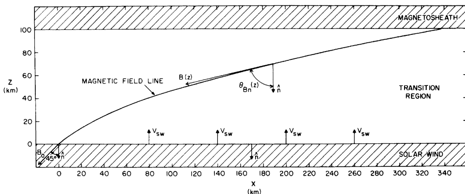
Fig. 2. The planar bow shock model when the upstream \theta_{Bn} is equal to 45^\circ . The shock transition region extends for 100 km in the \hat{z} direction and separates the upstream solar wind from the downstream magnetosheath. The magnetic field magnitude and electron concentration are assumed to increase linearly with increasing z . Within the shock transition region the plasma flow velocity is taken to be in the \hat{z} direction, and the plasma flux is constant. Because of the planar geometry the normal component of the magnetic field is constant throughout the transition region. A magnetic field line is shown, as is \theta_{Bn} near the center of the transition region.
