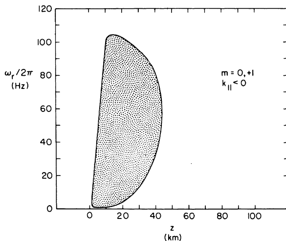
Fig. 5. The unstable frequencies as a function of shock penetration for the model distribution and generation via the Landau and anomalous cyclotron resonances. It is usually true that for a given frequency a wide range of wave normal angles is unstable. The distribution is stable for z greater than about 50 km because (k_{\parallel}/|k_{\perp}|)(\partial F/\partial v_{\parallel}) evaluated at the Landau resonance velocity is not sufficiently positive.
