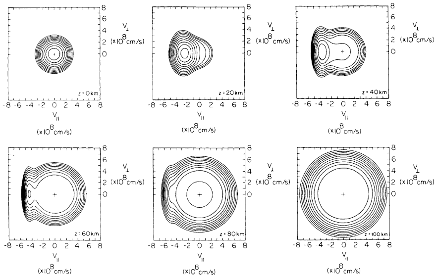
Fig. 3. Contour plots of the logarithm of the model electron velocity distribution as a function of shock penetration z . The distribution evolves from a relatively cool Maxwellian at the solar wind ( z = 0 km) to a relatively hot modified Lorentzian at the magnetosheath ( z = 100 km). As the beam energy increases, the anisotropy ratio T_{\perp}/T_{\parallel} increases, as does the modified Lorentzian component of the model distribution.
