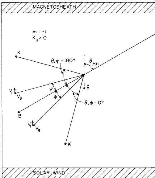
Fig. 6. Relative orientations of the magnetic field vector, the wave vector, the group velocity, and the plasma flow velocity for generation via the normal cyclotron resonance. All vectors lie in the plane of the figure. For a given wave normal angle the two wave vectors that lie in the plane of the planar bow shock model are distinguished by the angle \phi with the \phi = 0^\circ direction defined to be toward the solar wind. The \phi = 180^\circ orientation lies on the unstable cone of wave vectors and is 180^\circ in azimuth from the \phi = 0^\circ orientation. For a given wave vector orientation the ray path direction in the shock frame of reference is in the direction of the vector \mathbf{v}_g + \mathbf{v}_r . For k_{\parallel} > 0 , most of the ray paths are directed toward the solar wind. However, the \phi = 180^\circ orientation of \mathbf{k} together with the plasma convection effect can result in a ray path directed nearly transverse to the shock normal.
