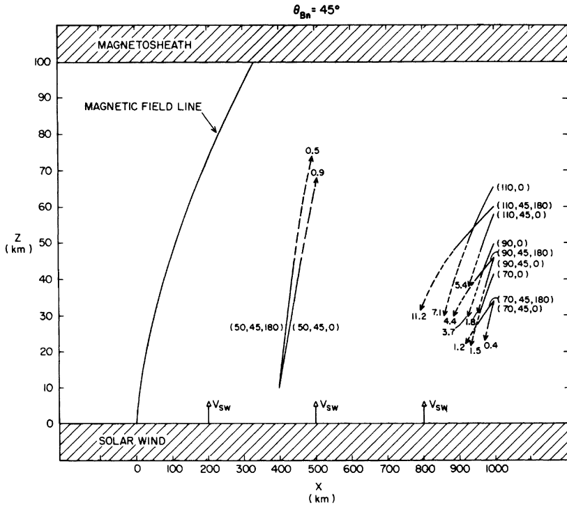
Fig. 8. Results of the propagation and integrated growth calculations when the upstream \theta_{Bn} is equal to 45^\circ . Shown are a magnetic field line and several ray paths in the shock transition region. The ray paths for generation via the Landau and anomalous cyclotron resonances originate in the lower left corner of the figure, while those for generation via the normal cyclotron resonance originate on the right side of the figure. The ray paths are labeled in the format (\omega_r/2\pi, \theta_0, \phi) where \theta_0 and \phi specify the initial wave vector orientation. A \phi value for \theta_0 = 0^\circ is not applicable and so is omitted from the ray path labels. The solid portions of the ray paths correspond to regions of growth, while the dashed portions correspond to regions of damping. At the heads of the arrows denoting the ray path, the maximum integrated growth along the ray path is given. The ray paths terminate when the integrated growth rate becomes negative. It is evident that some of the waves generated via the normal cyclotron resonance attain large amplitudes within the shock.
