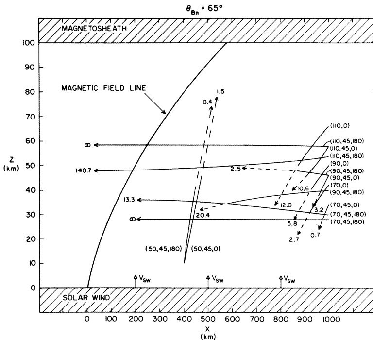
Fig. 9. Results of the propagation and integrated growth calculations when the upstream \theta_{Bn} is equal to 65^\circ . The format of the figure is similar to Figure 8. A comparison of Figure 8 and this figure suggests that the number of wave packets that attain large amplitudes within the shock increases with increasing \theta_{Bn} . The largest integrated growth occurs for waves that travel transverse to the shock normal.
