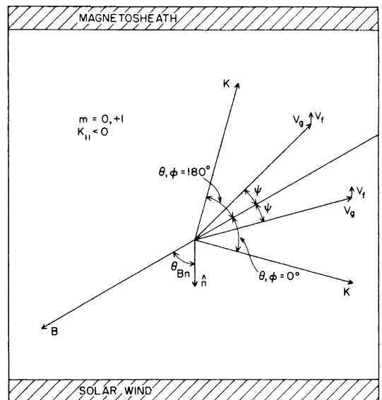
Fig. 7. Similar to Figure 6 but illustrating the geometry for the case of generation via the Landau and anomalous cyclotron resonances. The ray path directions in the shock frame are given by the direction of the vector \mathbf{v}_g + \mathbf{v}_r . In all cases, the ray paths are directed toward the magnetosheath.
