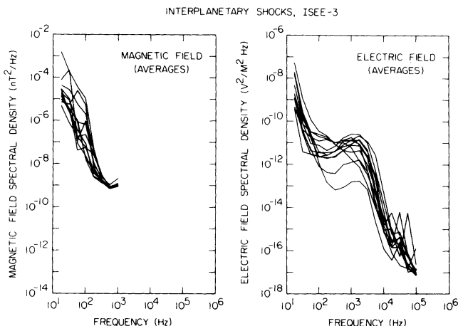
Fig. 5. Representative electric and magnetic field spectrums for a series of interplanetary shocks observed by ISEE 3 at 1 AU.
