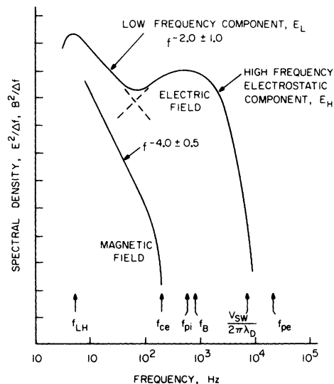
Fig. 3. A schematic representation of electric and magnetic field spectrums observed in the earth's bow shock.
