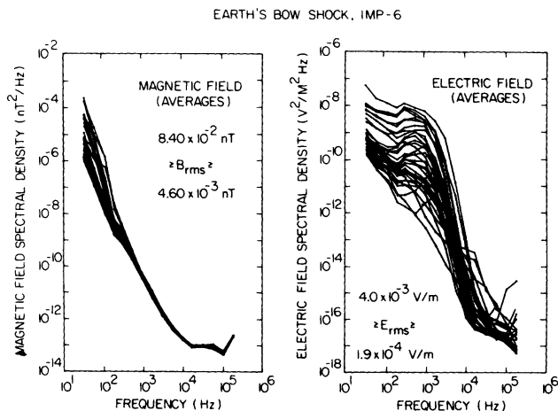
Fig. 2. Measured electric and magnetic field spectrums of plasma waves in the transition region of the earth's bow shock [from Rodriguez and Gurnett, 1975].
