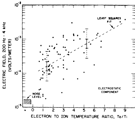
Fig. 6. A scatter plot showing the variation in the intensity of the high-frequency electrostatic noise as a function of the electron to ion temperature ratio [from Rodriguez and Gurnett, 1976].
