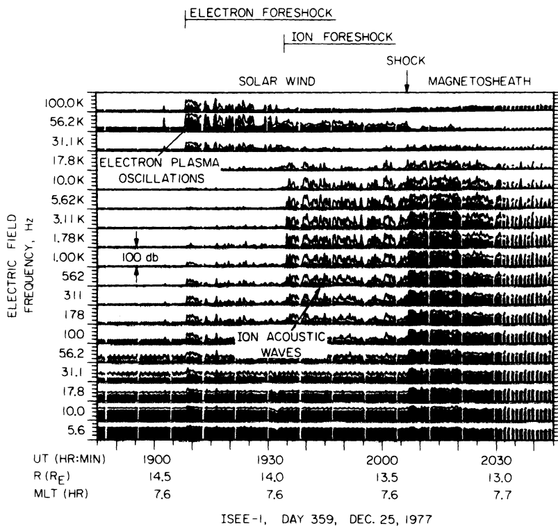
Fig. 11. A multichannel electric field plot showing the onset of electron plasma oscillations at the electron foreshock and the onset of ion acoustic waves at the ion foreshock.
