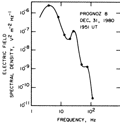
Fig. 9. A spectrum from Prognoz 8 showing a peak in the low-frequency electric field noise near the lower hybrid resonance frequency [from Vaisberg et al. , 1983].
