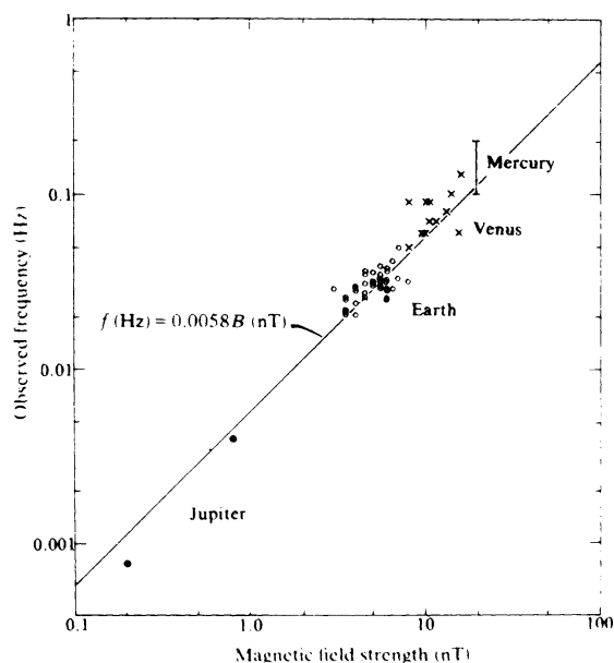
Fig. 16. The frequency of upstream ULF waves as a function of the ambient magnetic field strength at four planets: Mercury, Venus, the earth, and Jupiter [from Hoppe and Russell , 1982]. The frequency is typically about one-tenth of the proton cyclotron frequency.
