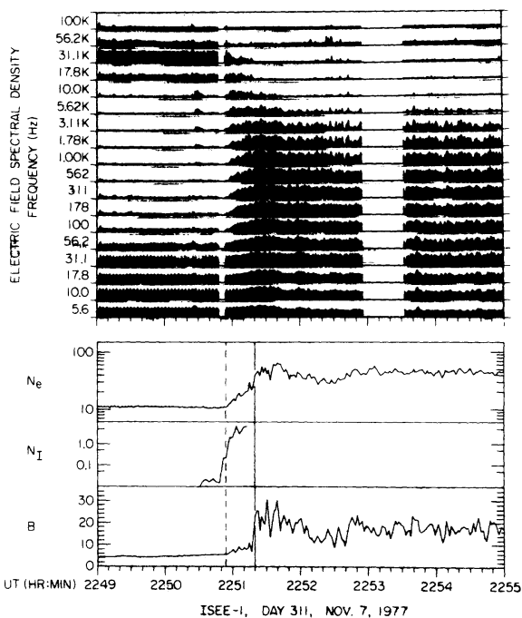
Fig. 7. Electric field and plasma measurements of a quasi-perpendicular shock from ISEE 1 showing that the onset of the high-frequency electrostatic noise occurs coincident with the onset of ions ( N_r ) gyrating ahead of the shock (plasma data from Paschmann et al. [1982] ).
