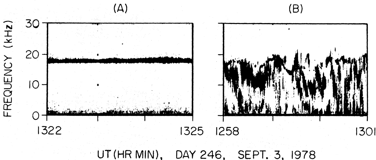
Fig. 12. High-resolution frequency-time spectrograms showing the change in the spectrum of electron plasma oscillations from (a) a very narrow-band emission near the electron foreshock boundary to (b) a much broader highly structured emission deep in the foreshock [from Fuselier et al., 1985].
