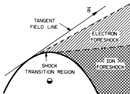
Fig. 10. An illustration showing the geometric relationship between the shock transition region, the tangent field line, and the electron and ion foreshock regions.
