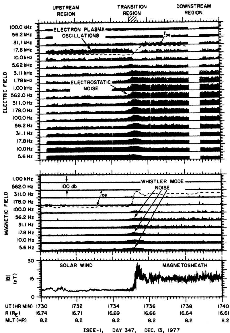
Fig. 1. A multichannel electric and magnetic field plot showing typical plasma wave intensities observed near the earth's bow shock.
