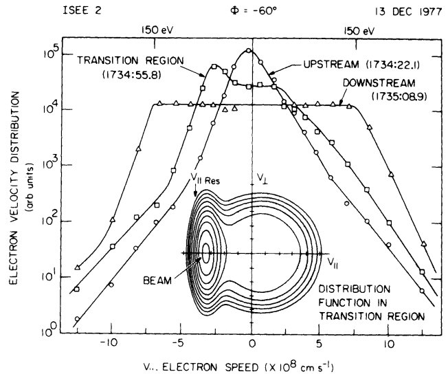
Fig. 8. A series of v_{||} cuts of the electron velocity distribution function obtained in the vicinity of the earth's bow shock. Note the beam in the transition region (plasma data from Feldman et al. [1982] ).
