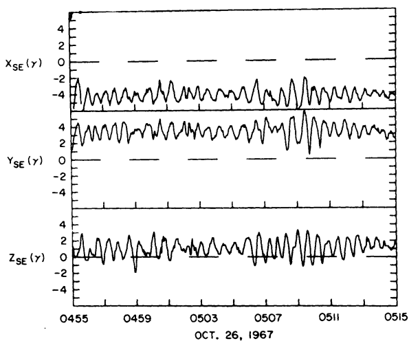
Fig. 15. An example of the magnetic fluctuations associated with the upstream ULF magnetohydrodynamic waves. Note the highly coherent nature of these waves and the large amplitude relative to the background field [from Fairfield , 1969].
