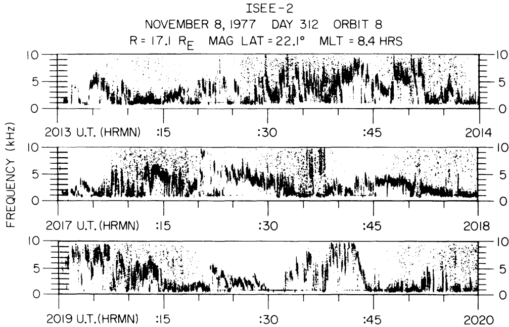
Fig. 14. High-resolution frequency-time spectrograms of ion acoustic waves observed in the ion foreshock region of the earth's bow shock [from Anderson et al. , 1981].
