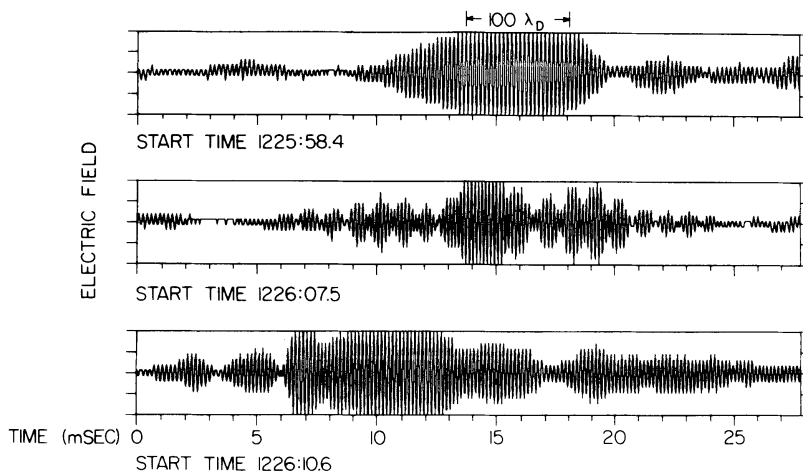
Fig. 13. Examples of solitonlike structures in the waveform of electron plasma oscillations observed upstream of Jupiter's bow shock [from Gurnett et al. , 1981a].
