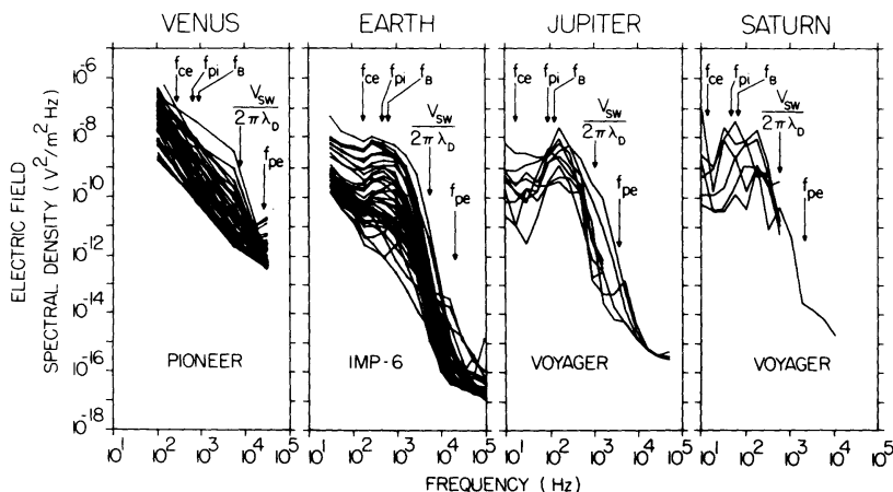
Fig. 4. A comparison of the transition region electric field spectrums from four planets: Venus, the earth, Jupiter, and Saturn.
