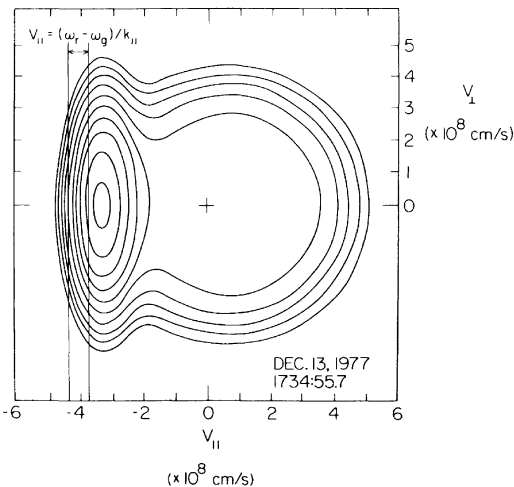
Fig. 4. In this figure, the range in the m = -1 cyclotron resonance velocity corresponding to instability for \omega_r/2\pi = 110 Hz, as obtained from Figure 2, is overlaid on a contour plot of the electron distribution function measured on December 13, 1977, at 1734:55.7 UT. The m = -1 cyclotron resonance velocities lie in regions of large anisotropy, \partial F/\partial\alpha < 0 .
