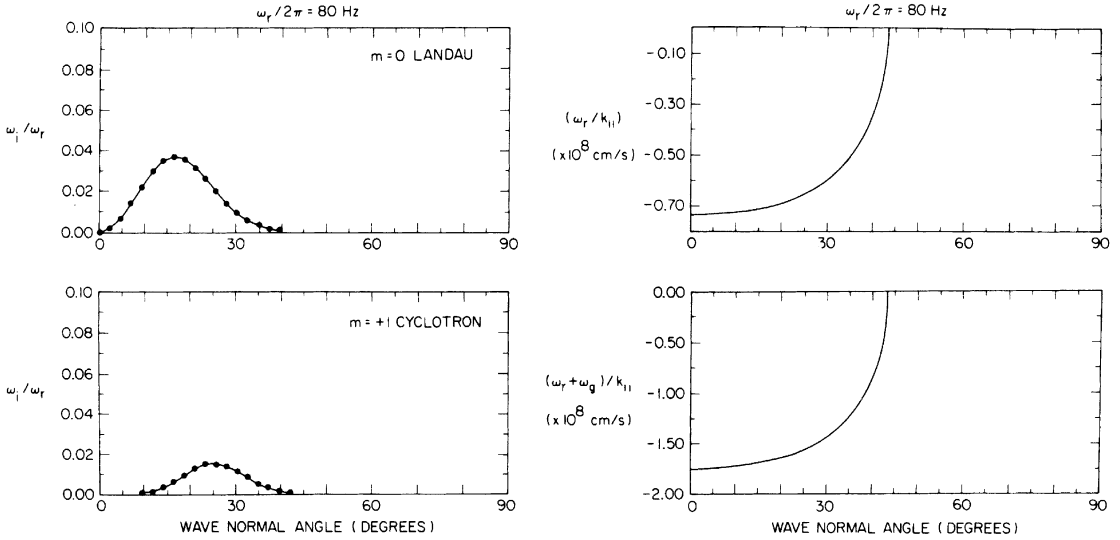
Fig. 5. The left column of this figure presents a sample of the growth rates obtained for the electron distribution function measured on October 15, 1978, and for the frequency \omega_r/2\pi = 80 Hz. The unstable waves have k_{\parallel} < 0 , corresponding to wave vectors directed toward the magnetosheath. The top left panel shows the m = 0 Landau contribution to the growth rate, while the bottom left panel shows the m = +1 cyclotron contribution to the growth rate. For this frequency and these wave normal angles the m = -1 cyclotron contribution to \omega_i/\omega_r are negative and negligible. The right column depicts both the m = 0 Landau resonance velocity and the m = +1 cyclotron resonance velocity as a function of the wave normal angle.
