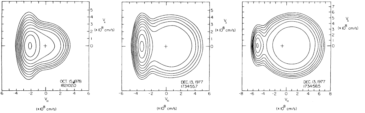
Fig. 2. This figure depicts contour plots of the logarithm of the analytic fits to the electron distribution function data analyzed in this study. These distribution functions were measured within the transition region of earth's bow shock. A modified Lorentzian models the flat-topped component of the electron distribution and a convected Maxwellian with a T_{\perp} < T_{\parallel} anisotropy models the field-aligned electron beam.
