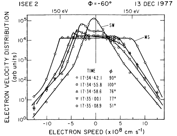
Fig. 1. This figure, reproduced from Feldman et al. [1982], shows parallel slices of electron distribution function data measured by the ISEE 2 fast plasma experiment. As the satellite moves from the solar wind into the magnetosheath, field-aligned electron beams are observed.
