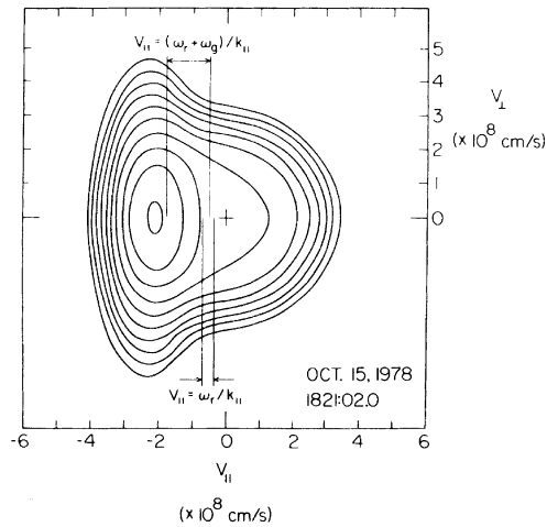
Fig. 6. In this figure, the range in the m = 0 Landau and the m = +1 cyclotron resonance velocities corresponding to instability for the case \omega_r/2\pi = 80 Hz, as obtained from Figure 4, is overlaid on a contour plot of the electron distribution function measured on October 15, 1978. The m = 0 Landau resonance velocities lie in regions of positive (k_{\parallel}/|k_{\parallel}|)(\partial F/\partial v_{\parallel}) , while the m = +1 cyclotron resonance velocities lie in a region of large anisotropy, \partial F/\partial \alpha > 0 .
