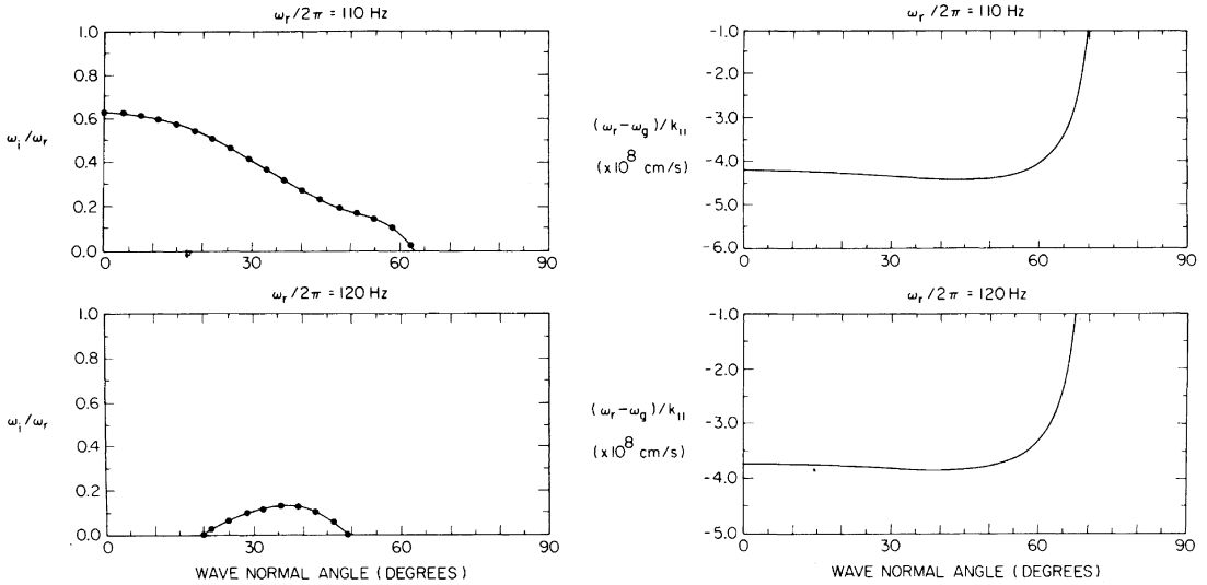
Fig. 3. The left column of this figure presents a sample of the growth rates obtained for the electron distribution function measured on December 13, 1977, at 1735:55.7 UT. Plotted is the ratio of the total growth rate to real frequency. These waves are generated by the m = -1 cyclotron resonance and have k_{\parallel} > 0 . The right column of this figure depicts the m = -1 cyclotron resonance velocity as a function of wave normal angle for the two frequencies of interest.
