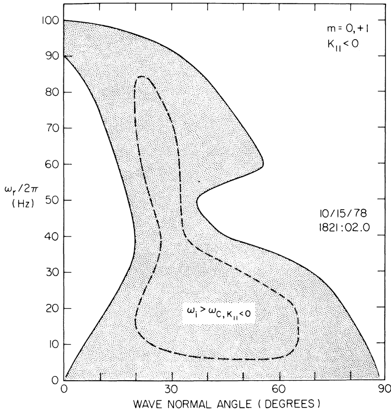
Fig. 7. This figure depicts the unstable frequencies and wave normal angles that are generated by the m = 0 and +1 resonances for the electron distribution function measured on October 15, 1978. The waves have k_{||} < 0 , corresponding to wave vectors directed toward the magnetosheath. The largest growth rates lie in the shaded region bounded by the dashed line.
