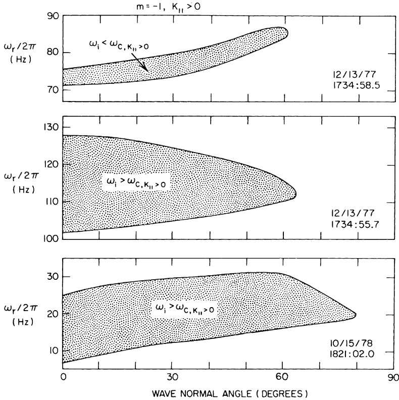
Fig. 8. This figure depicts the unstable frequencies and wave normal angles that are generated by the m = -1 cyclotron resonance for the electron distribution functions shown in Figure 2. All of the waves have k_{||} > 0 , corresponding to wave vectors directed toward the solar wind. The growth rates for the distribution measured at 1734:58.5 UT on December 13, 1977, are smaller than the critical growth rate.
