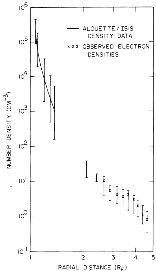
Fig. 12. A log-log plot comparing low-altitude median electron densities obtained from the topside sounder data of Alouette II and ISIS 1 and high-altitude median electron densities obtained from the PWI on DE 1.
