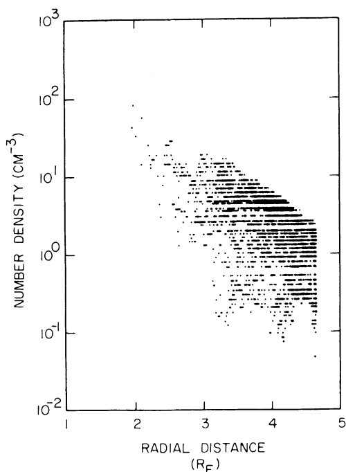
Fig. 9. A scatter plot of electron density as a function of radial distance. The large scatter in the data is mainly due to temporal variations in the electron density. The sharp upper cutoff evident from about 3.5 to 4.6 R_E is caused by the whistler mode propagation cutoff at the electron gyrofrequency.
