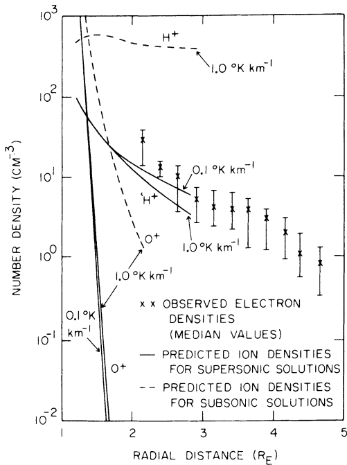
Fig. 11. Predicted ion densities below 2.8 R_E based on solutions to the 13-moment transport equations [Schunk and Watkins, 1982]. The subsonic outflow solutions correspond to higher H^+ and O^+ densities. These predicted densities exceed the DE 1 measured densities at 2 R_E by more than an order of magnitude. Supersonic outflow solutions correspond to lower H^+ and O^+ densities. An increase in the boundary electron temperature gradient (from 0.1^\circ K km^{-1} to 1^\circ K km^{-1} ) corresponds to a slight increase in the predicted O^+ densities and a larger decrease in the predicted H^+ densities. Both sets of predicted ion densities for the supersonic outflow solutions are within 25% of the median density values observed by DE 1.
