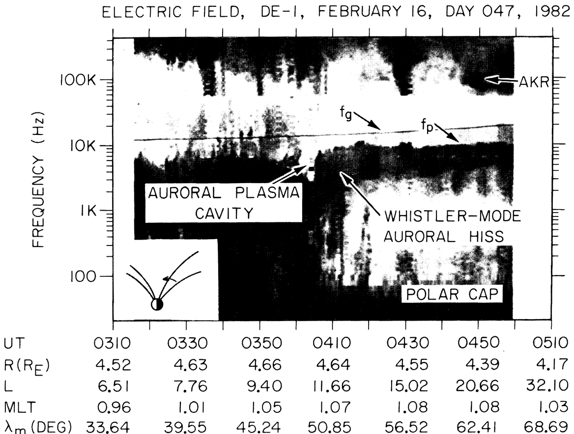
Fig. 4. A nightside crossing of the auroral field lines in mid-February illustrating a depletion in electron densities at \lambda_m \approx 50^\circ [Calvert, 1981] and a smooth density profile inside the polar cap region.
