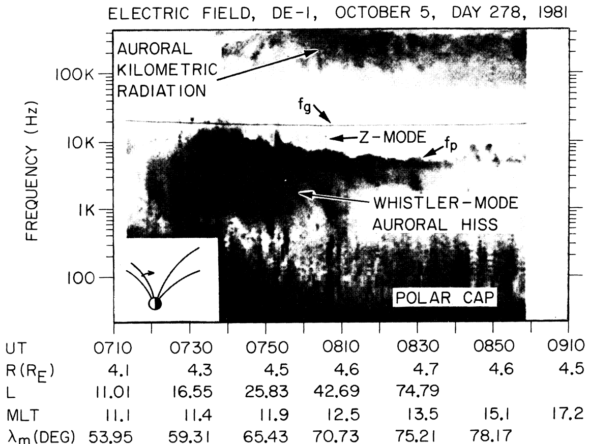
Fig. 3. An electric field spectrogram of a polar cusp crossing in early October. Irregularities in the density profile are indicated by sudden increases in f_p at 0752 UT and at 0845–0850 UT as the satellite nears the pole.
