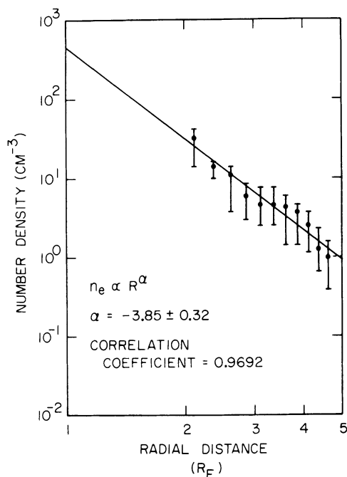
Fig. 10. A log-log plot of median number densities as a function of radial distance. The best line fit through these points indicates a power law distribution for electron densities in the polar cap: n_e \propto R^{-3.85} .
