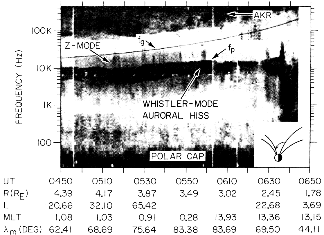
Fig. 5. A continuation of the same polar pass illustrated in Figure 4. The density profile is smoothly varying over the entire polar cap region.
