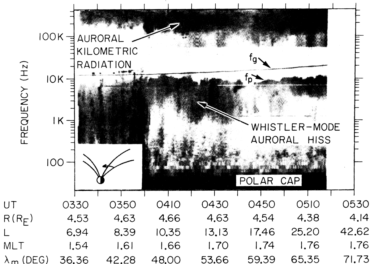
Fig. 7. Another nightside crossing of the auroral field lines in early February. Changes in the cutoff frequency for this pass indicate small variations in the number density by a factor of 2 or less.
