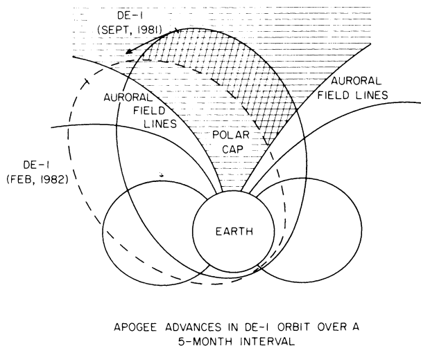
Fig. 1. The change in the orientation of the DE 1 orbit from September 1981 to February 1982. All density data presented in this study for the 5-month interval, indicated by the crossing shading, are from high-latitude passes over the polar cap region.
