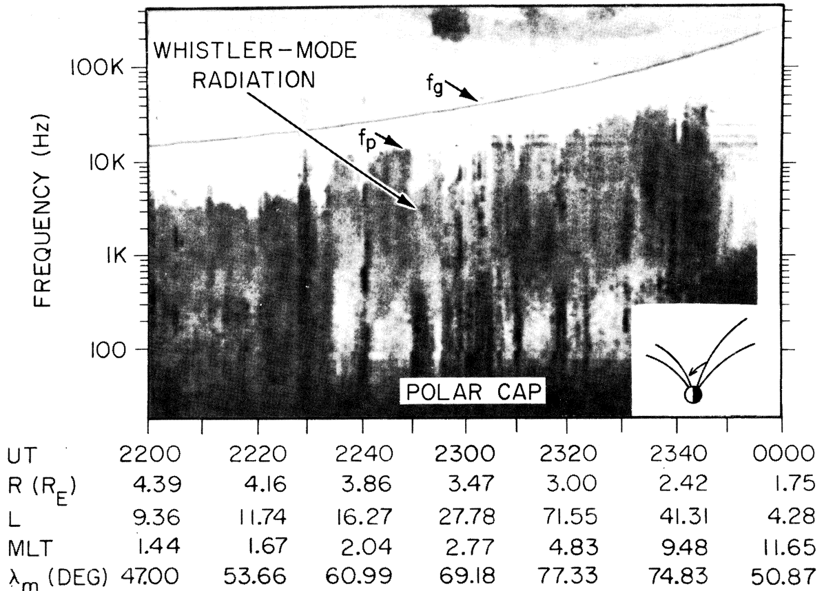
Fig. 6. A spectrogram illustrating the time variability of the density profile. This pass preceded the pass illustrated in Figures 4 and 5 by just 6 hours for the same region of the polar magnetosphere. The density profile is highly variable on very short spatial scales.
