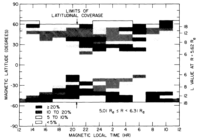
Fig. 13. The frequency of occurrence of the broad-band electrostatic noise as a function of magnetic latitude and magnetic local time in the region from 5.01 to 6.31 R_E [from Gurnett and Frank , 1977]. In contrast to the ULF-ELF magnetic noise the broad-band electrostatic noise occurs at all local times and is not uniquely related to the polar cusp region, even though it occurs in the cusp.
