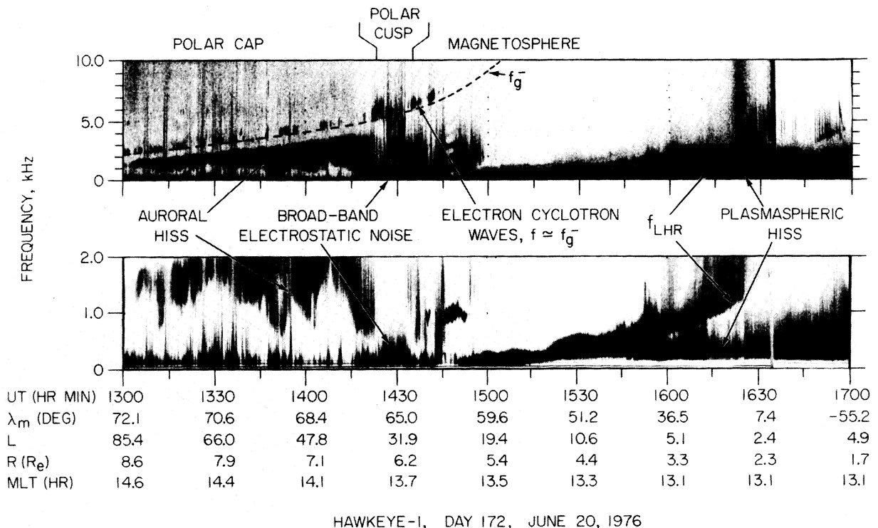
Fig. 5. High-resolution frequency-time spectrograms showing further details of the electric field emissions detected during the polar cusp crossing in Figure 1. The low-frequency component, \leq 2.0 kHz, of the broad-band electrostatic noise is clearly evident in the polar cusp. Whistler mode auroral hiss emissions, with a sharp upper-frequency cutoff slightly below the electron gyrofrequency f_g^- can be seen propagating into the region on the polarward side of the cusp. Electrostatic electron cyclotron waves at f \approx f_g^- are also evident in the polar cap and magnetosphere.
