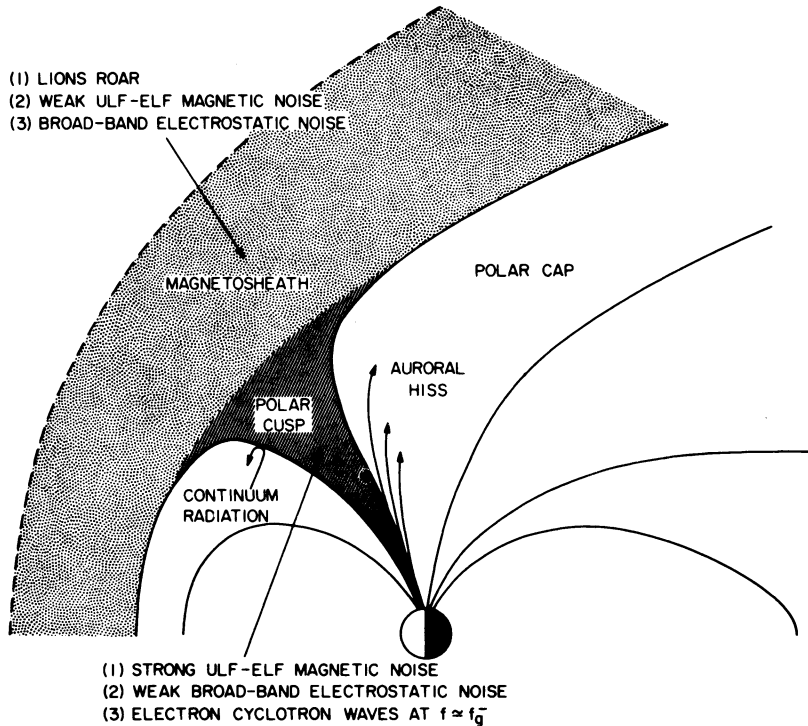
Fig. 15. A summary of the primary types of plasma wave phenomena observed in the polar cusp and the magnetosheath. Many of the plasma waves observed in these two regions are very similar. The main differences are that the lion's roar emissions do not occur in the polar cusp and that the electrostatic electron cyclotron waves are not observed in the magnetosheath.
