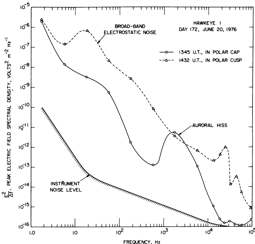
Fig. 6. Representative spectrums of the broad-band electrostatic noise and auroral hiss from Figure 1. The rms electric field strength of the broad-band electrostatic noise is about 4.8 \text{ mV m}^{-1} .
