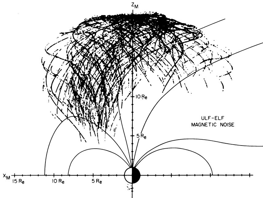
Fig. 11. The region of occurrence of the ULF-ELF magnetic noise in geomagnetic coordinates. Only events exceeding the receiver noise level (see Figure 8) by at least 10 dB from 1.78 to 56.2 Hz are shown. The ULF-ELF magnetic noise in both the magnetosheath and the polar cusp usually exceeds this threshold.
