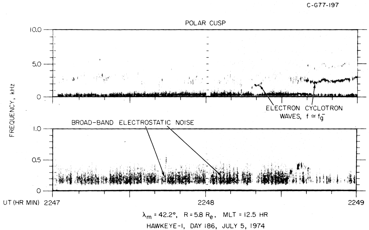
Fig. 14. Expanded time scale spectrograms of the electron cyclotron waves and broad-band electrostatic waves near the cusp-magnetosphere boundary in Figure 10. Within the cusp the electron cyclotron waves become very diffuse and poorly defined. The broad-band electrostatic noise is seen to consist of many impulsive bursts extending across a broad range of frequencies.
