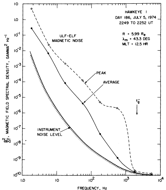
Fig. 8. A spectrum of the peak and average magnetic field strengths of the ULF-ELF magnetic field noise in Figure 3. Note the upper cutoff in the noise spectrum near the local electron gyrofrequency f_g^- . This cutoff suggests that the ULF-ELF noise consists of whistler mode waves.
