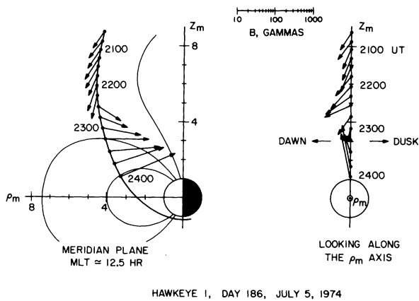
Fig. 7. The magnetic field directions and magnitudes for the pass in Figure 3. The magnetic fields are shown projected in a magnetic meridian ( \rho_m , Z_m ) plane through the spacecraft and in a plane perpendicular to the \rho_m axis. The Z_m axis is parallel to the magnetic dipole axis of the earth. In the polar cusp, from about 2225 to 2255 UT, the magnetic field has a strong dipolar component, with some skewing of the magnetic field out of the meridian plane toward local dawn.
