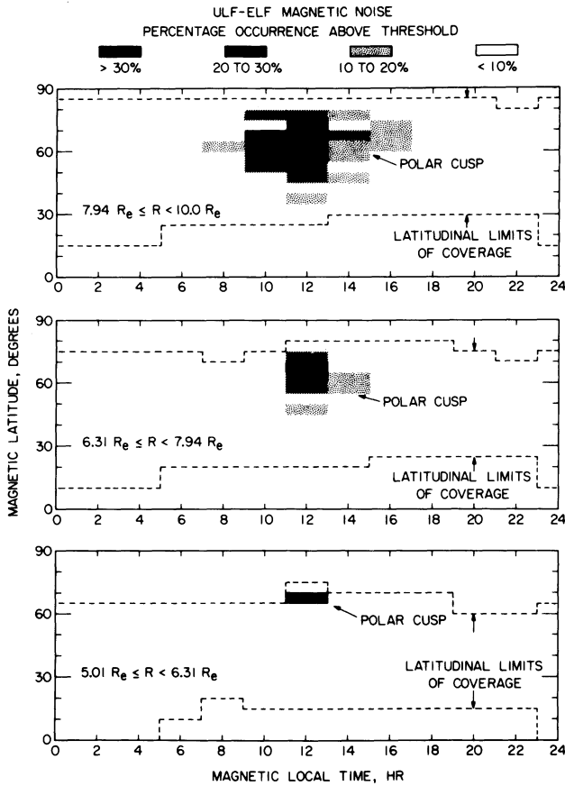
Fig. 12. The frequency of occurrence of the ULF-ELF magnetic noise as a function of magnetic local time and magnetic latitude within specific radial distance ranges. The general outline of the polar cusp region, decreasing in angular size with decreasing radial distance, is clearly evident.
