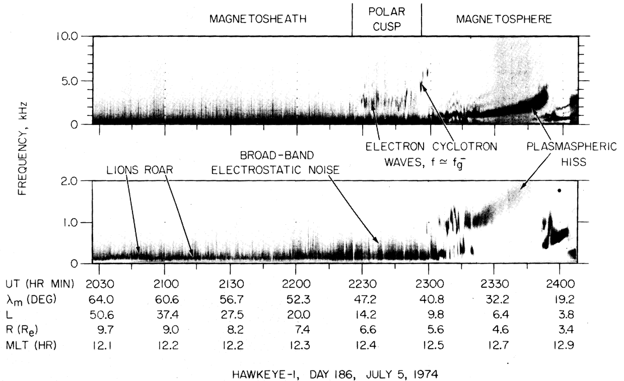
Fig. 10. High-resolution frequency-time spectrograms of the electric field emissions detected during the polar cusp crossing in Figure 3. The electrostatic electron cyclotron waves are seen to terminate near the cusp-magnetosheath boundary.
