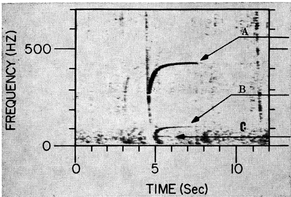
Fig. 1. Frequency-time spectrogram of a short fractional hop electron whistler followed, in order of decreasing frequency, by (A) a proton whistler at about 432 Hz, (B) a helium whistler at about 108 Hz, and (C) an 8-amu/unit charge whistler at about 54 Hz. Altitude is 1268 km, invariant latitude is 46.7°, and local time is 0.34 hr.
