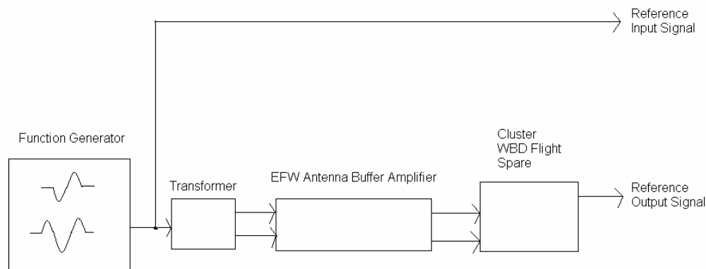
Figure 2. Block diagram of the Impulse Response Test Setup
