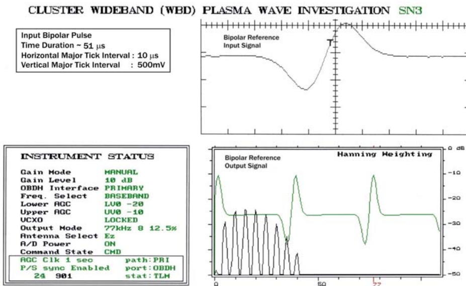
Figure 5. Example of Bipolar Pulse Input Reference Signal and Undistorted Bipolar Pulse Reference Output Signal in the 77 kHz Output Mode
