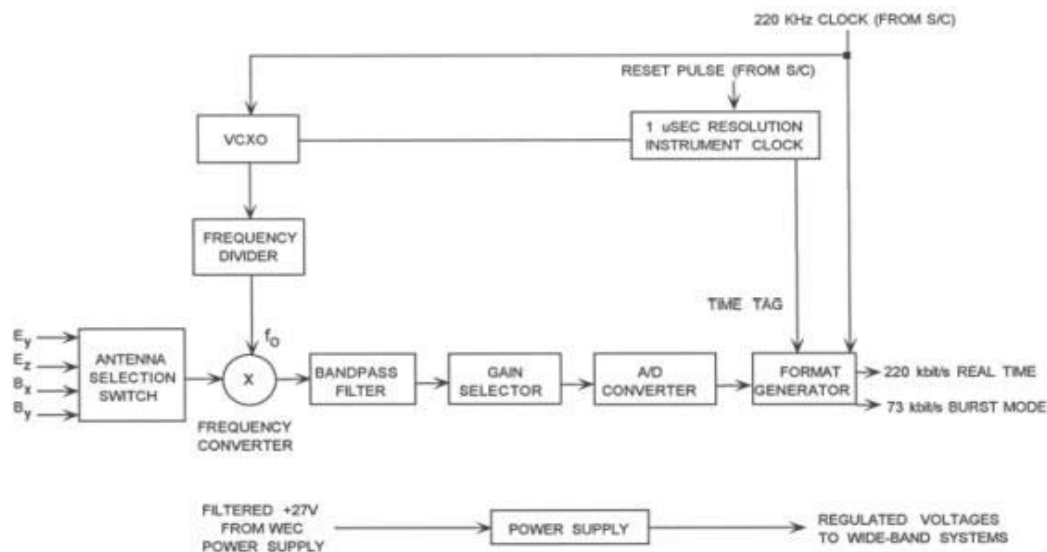
Figure 1. Block diagram of the WBD instrument.
