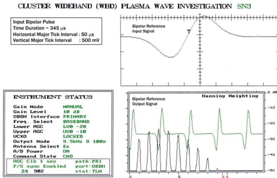
Figure 3. Example of Bipolar Pulse Input Reference Signal and Undistorted Bipolar Pulse Reference Output Signal in the 9.5 kHz Output Mode
