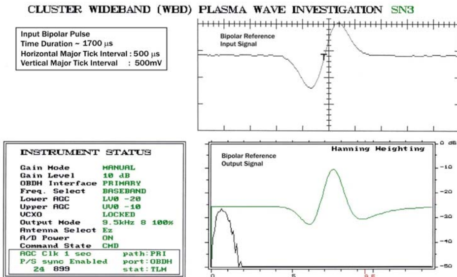
Figure 4. Example of Bipolar Pulse Input Reference Signal and Distorted Bipolar Pulse Reference Output Signal in the 9.5 kHz Output Mode
