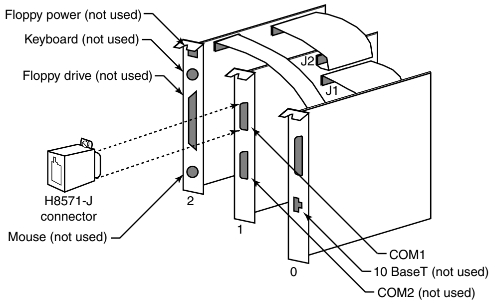
Figure 5-2 Connectors
