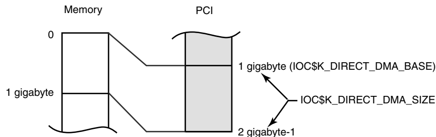
Figure 19-1 PCI-Based DMA
