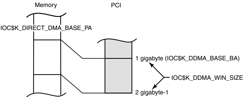
Figure 19-2 OpenVMS DMA
