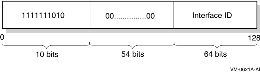
Figure 1–7 IPv6 Link-Local Unicast Address
