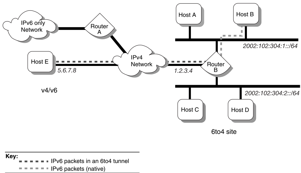
Figure 1–18 IPv6 Network-to-IPv6 Network Configuration over Tunnel
