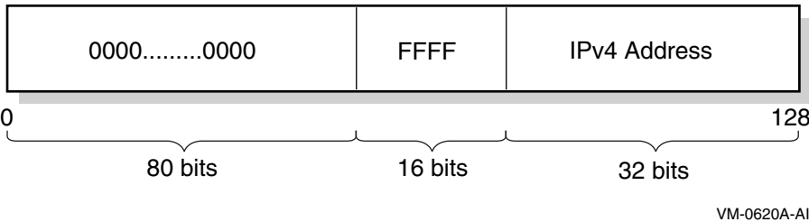
Figure 1–6 IPv4-Mapped IPv6 Address
