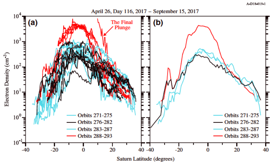
Figure 3. Panel (a) shows the latitudinal distributions of the Radio and Plasma Wave Science electron density measurements for all of the Grand Finale orbits. The latitudinal electron density profiles are color coded according to the altitude of Cassini at closest approach. These latitudinal profiles show strong variability from orbit to orbit, up to 2 orders of magnitude, as well as a significant north-south asymmetry due, in part, to the ring shadow effect in the southern hemisphere. Panel (b) shows the electron density measurements for the four groupings of the Grand Finale orbits averaged in latitude bins of 2^\circ . The averaged latitudinal electron density profiles show a strong altitude dependence within 10^\circ of the ring plane.
